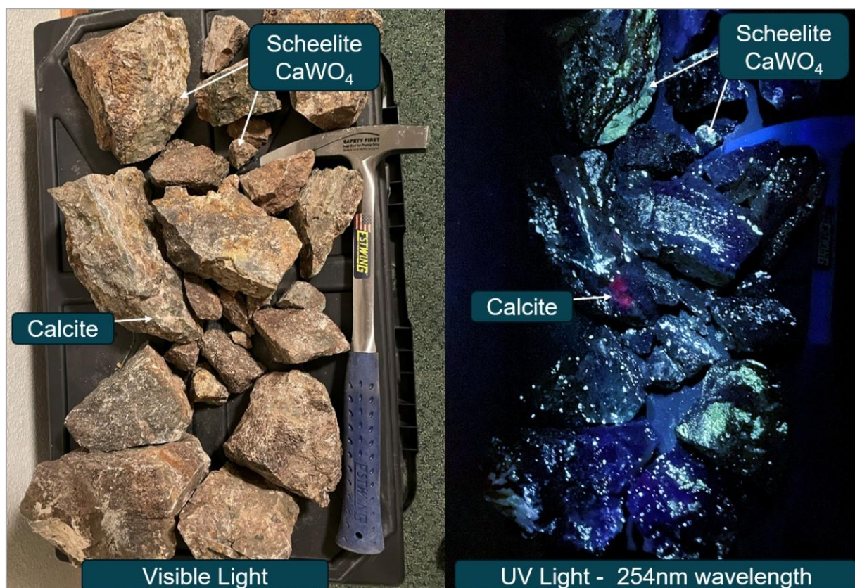
Figure 1; Photo of LKMET0004 metallurgical grab samples collected from the Linka Project Open Pit shown in visible and UV light. Dominant fluorescent mineral (white/blue colour) is scheelite. Sample shown is part of larger 58kg sample which assays 1.3%WO 3 .
