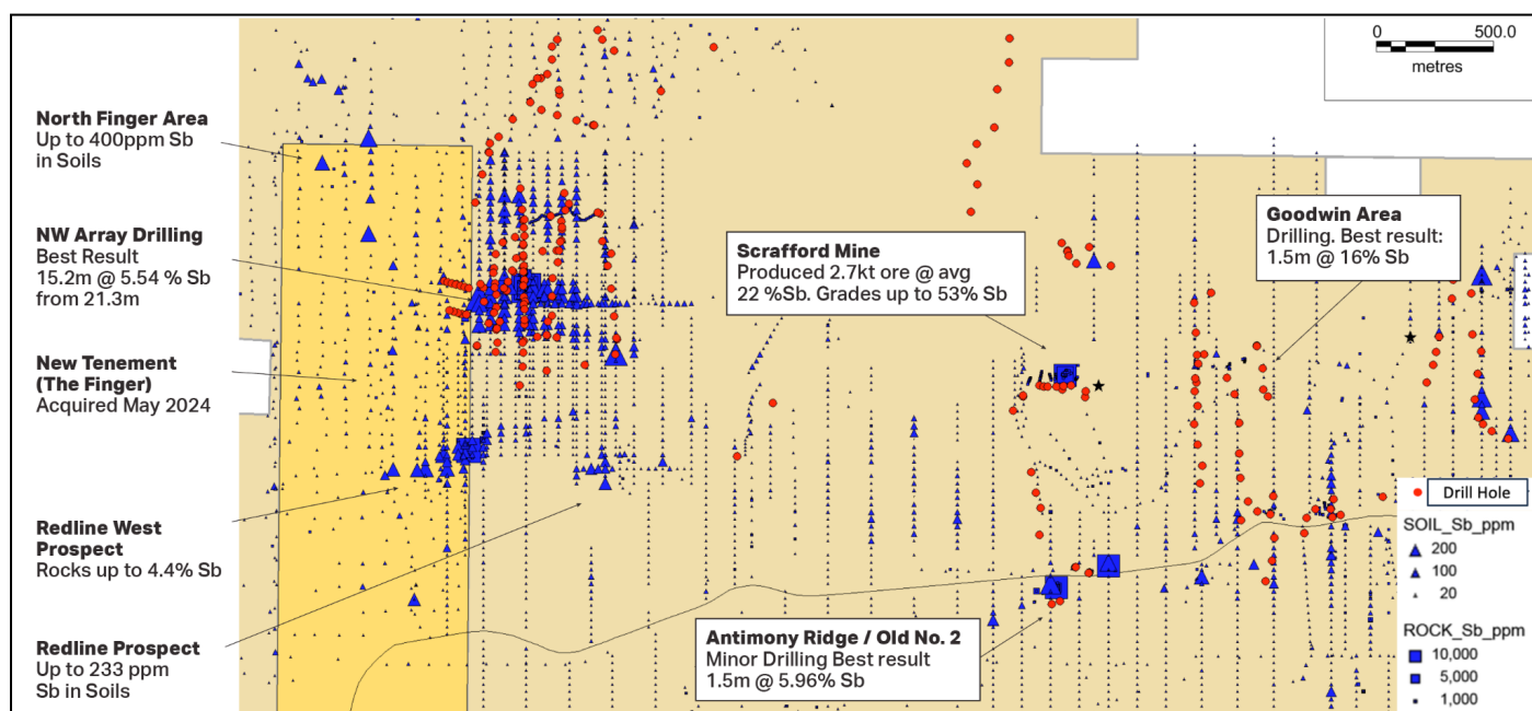
Fig. 4 Sb in Soils and Rocks with Drill Collars around the Scrafford Sb Mine
