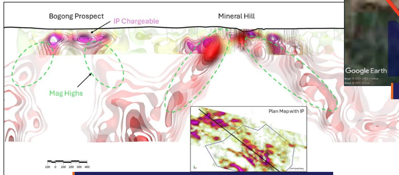
Long section at the Bogong Prospect – magnetics and IP anomalies 1 .
