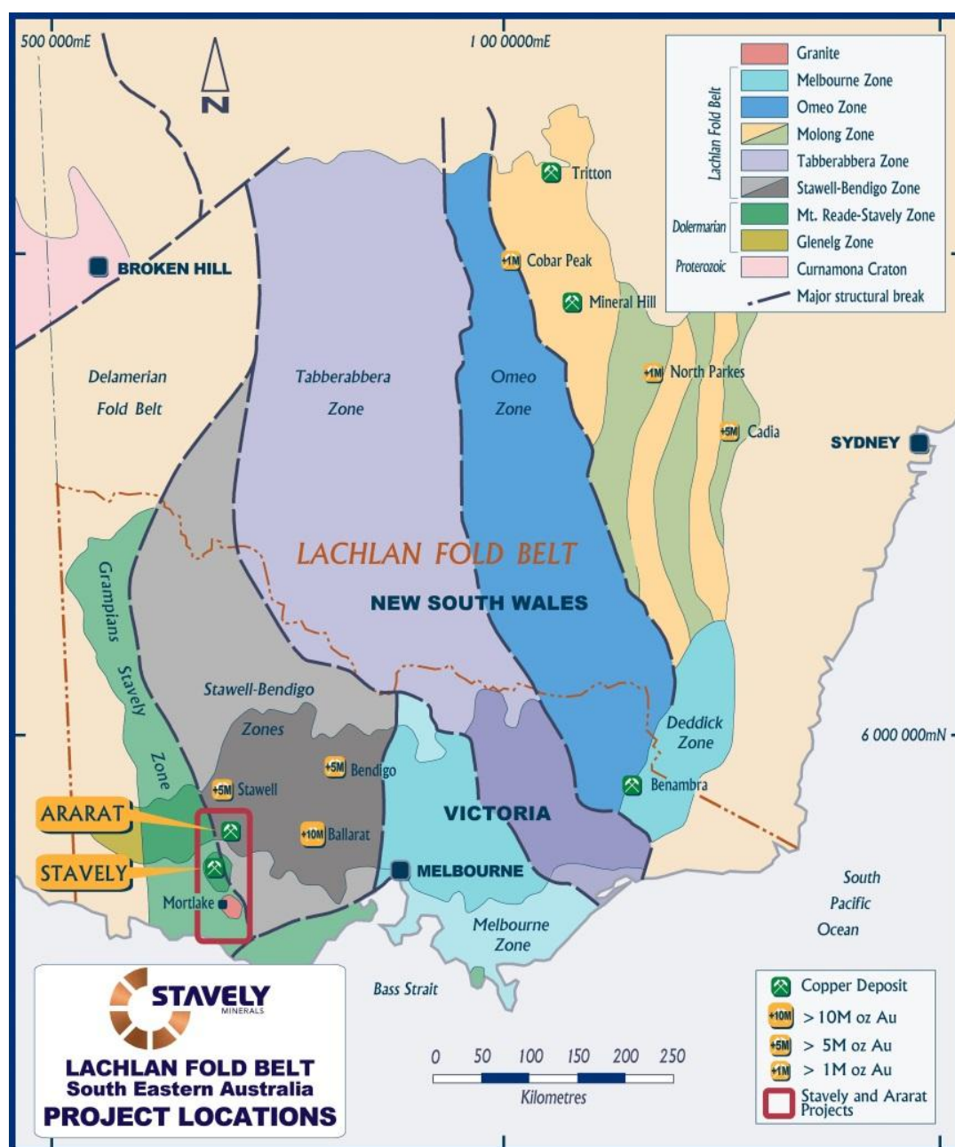
Figure 2. Geology of South-eastern Australia.
