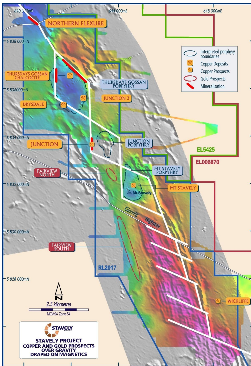
Figure 7. A portion of the Stavelly structural trend showing the location of several significant copper prospects – the Toora Road prospect to the north and the S2 and S3 porphyry prospects to the south are not shown on the extent of this figure. Coloured gravity draped on grey-scale 1VD magnetics.
