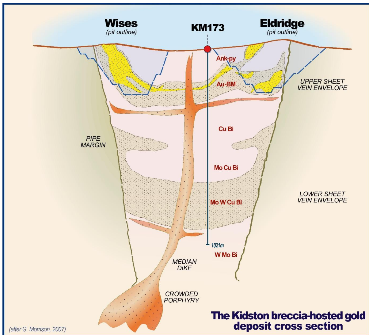
Figure 28. Cross- section of the Kidston breccia-hosted gold deposit showing the distribution of gold mineralisation (yellow) associated with a vertical metals zonation. Note that gold mineralisation is spatially restricted and associated with specific phases of brecciation and mineralisation. (Au-BM = gold and base metals, Ank-py = ankerite and pyrite) (After G. Morrison, 2007).
