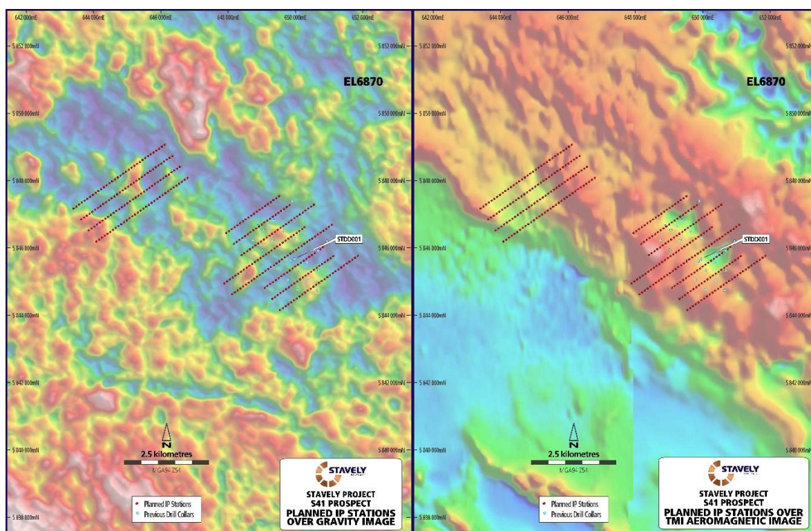
Figure 26. S41 gold prospect over gravity image (left) and aeromagnetic image (right) with planned IP Stations.
