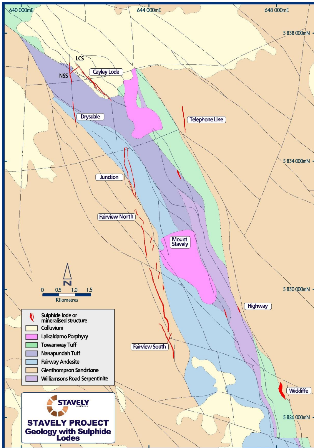
Figure 14. Stavely Project – Cayley Lode to Fairview South Prospect Location Plan.
