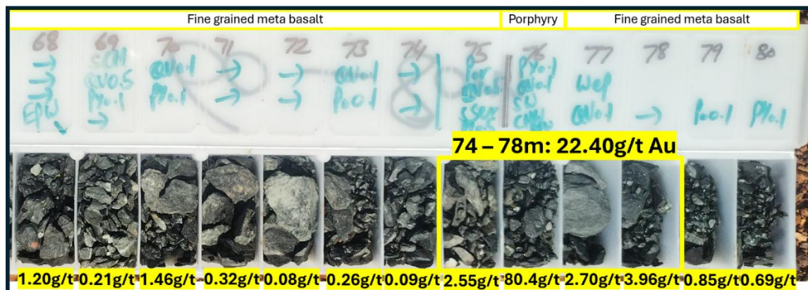
Figure 5: Pericles Chip Tray (LSRC24014) highlighting gold mineralisation including 4m @ 22.40g/t Au from 74m
