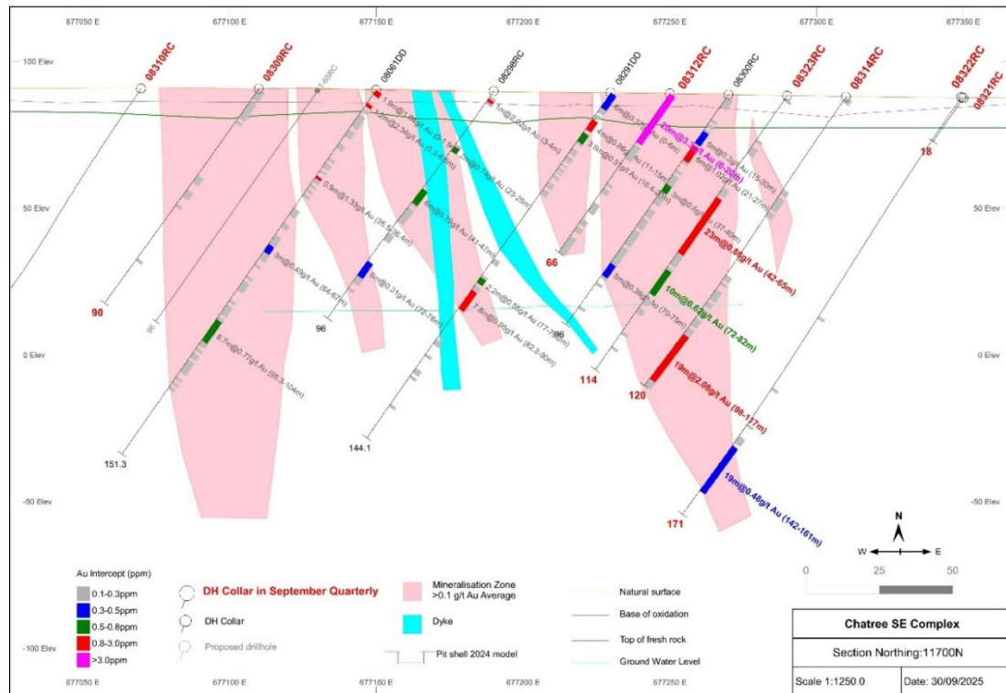
Figure 3: Significant Au intercepts 19 in section 11700N, T prospect.
