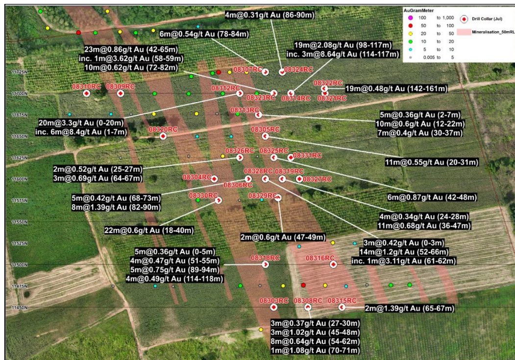
Figure 2: Drill hole locations 17 and significant intercepts 18 at T Prospect, Chatree South-East Complex.
