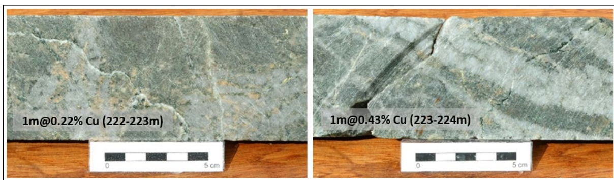
Figure 4: Phyllic altered porphyritic diorite with quartz veins (222-224m), Singto prospect.
