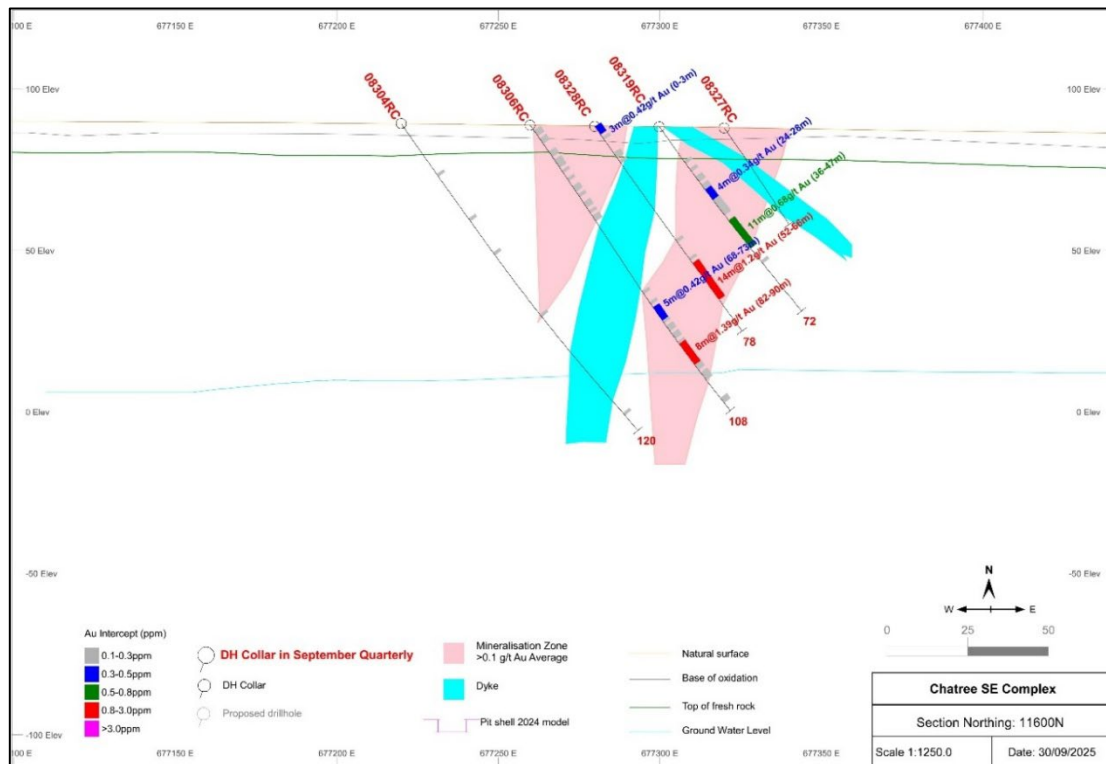
Figure 4: Significant Au intercepts 20 in section 11600N, T prospect.
