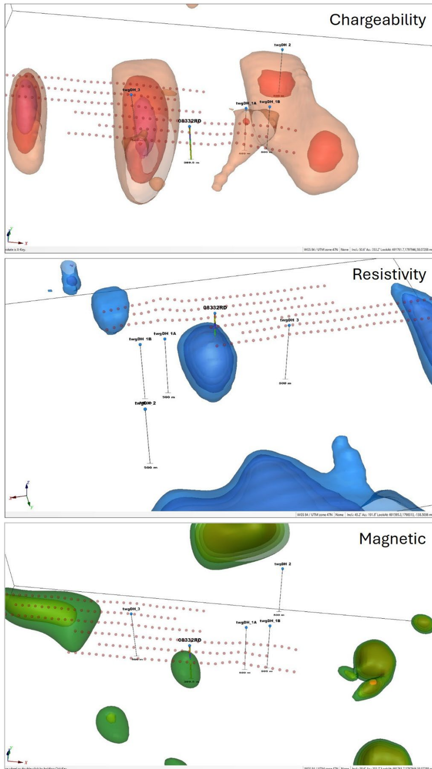
Figure 5: Deep drilling planned for geophysical targets from 3-dimensional models.
