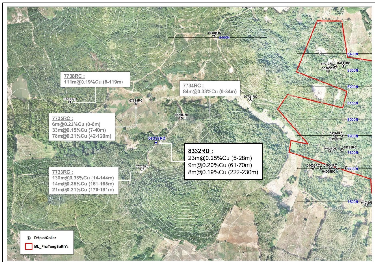
Figure 3: Drillhole locations, Singto Prospect 22 .
