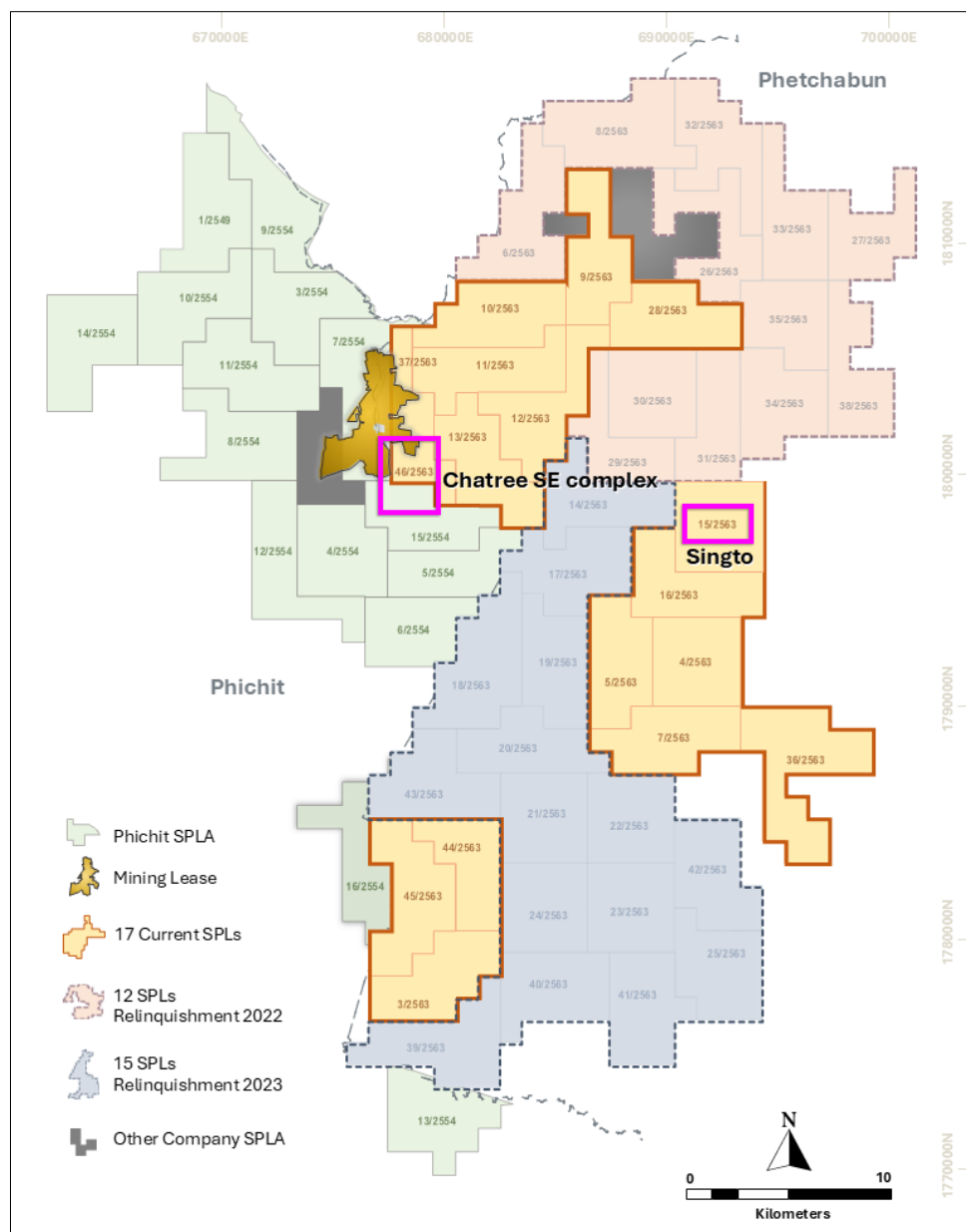
Figure 1: Chatree South-East Complex and Singto Prospect Locations 15 .
