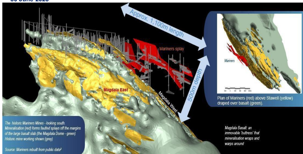
Figure 4 The historic Mariners Lodes occur above the Stawell basalt and are characteristic compared to Stawell-type mineralisation, including abundant visible gold. The Mariners system had historic production of 0.78-0.95Moz Au at grades of 28-30 g/t Au. Identifying repeats of Mariner-type mineralisation is an exciting target style for NSM exploration.
