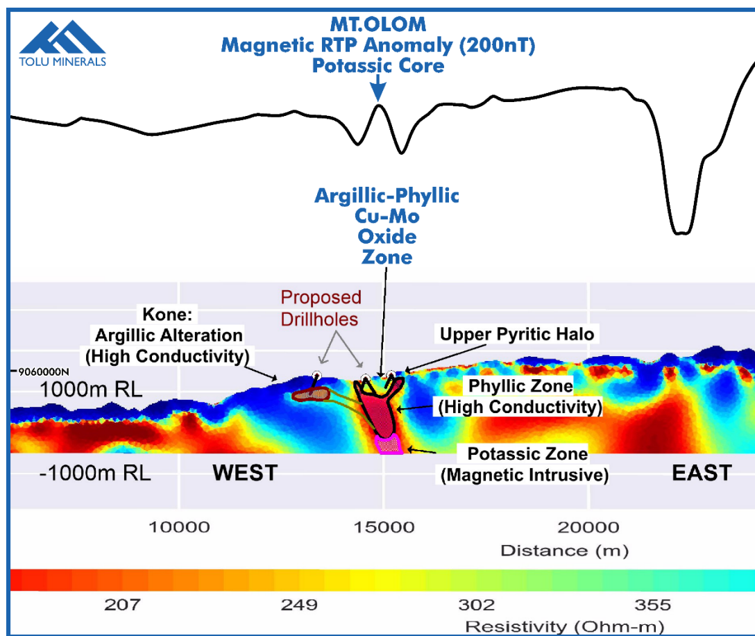
Figure 3: Airborne MT Resistivity Cross-Section (L-720)
