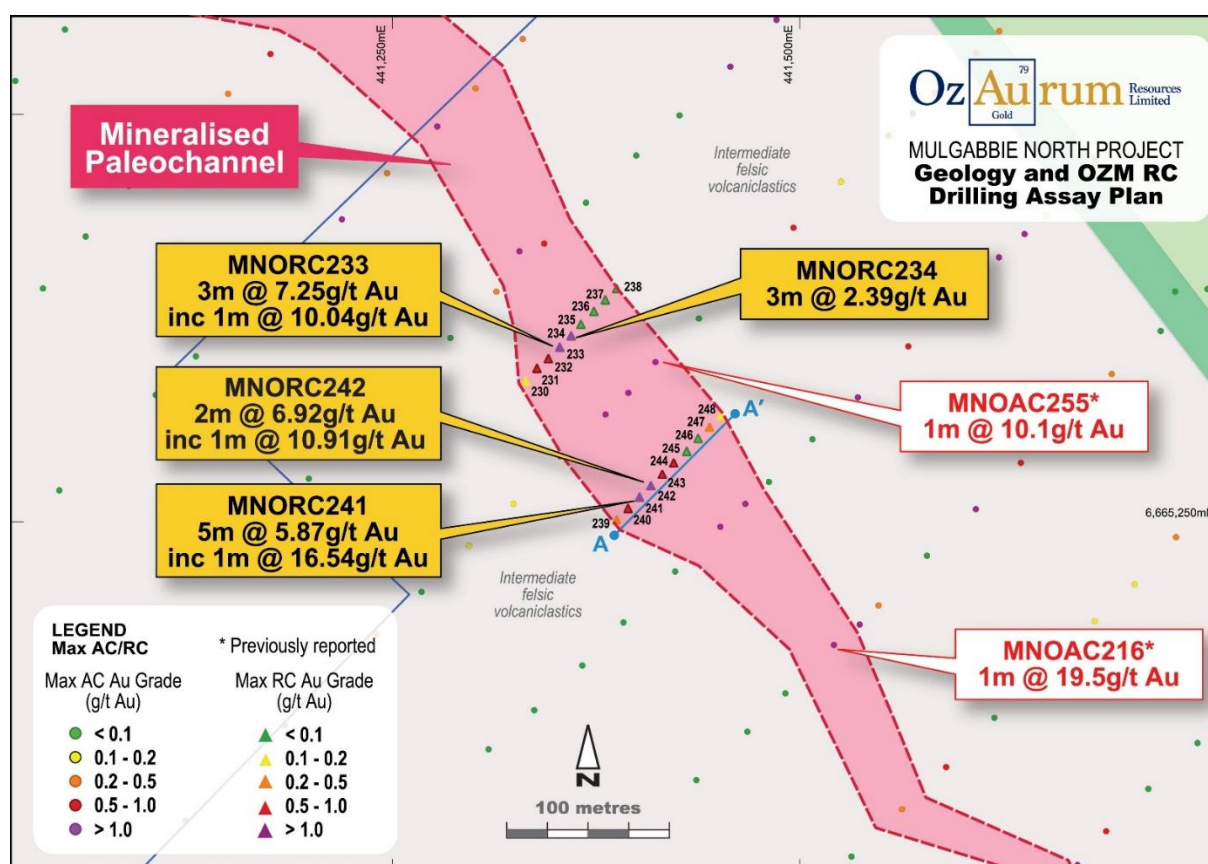
Figure 7: Paleochannel drill hole location plan Mulgabbie North
