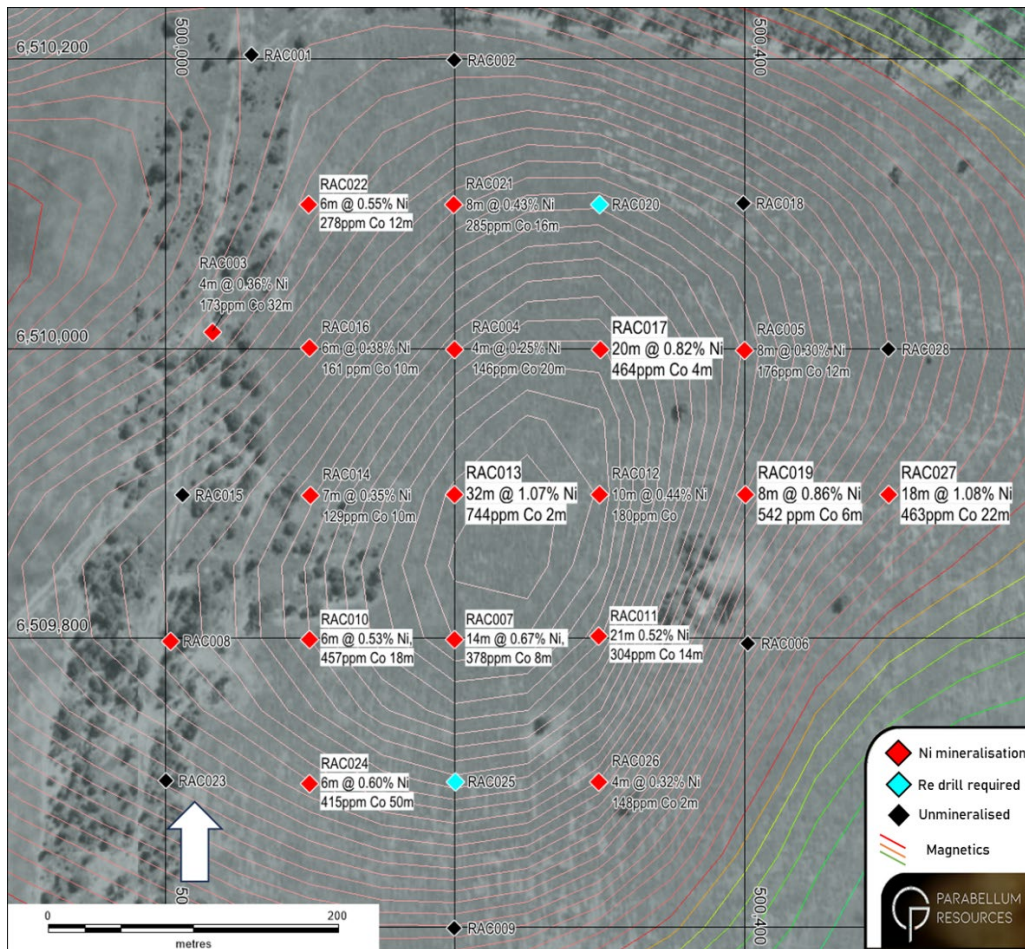
Figure 4: Redlands Prospect – Aircore drilling: Significant and anomalous nickel results (Source PBL 4 th December 2023)
