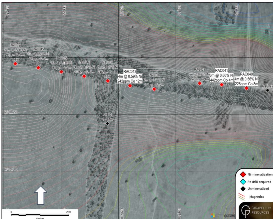
Figure 6: Redlands Prospect West – Aircore drilling: Significant and anomalous nickel results (Source PBL 4 th December 2023)
