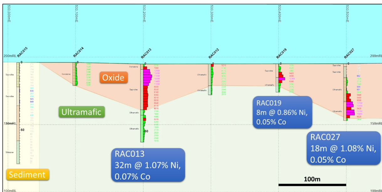
Figure 5: Redlands Prospect– Section 6,509,900mN (Source PBL 4 th December 2023)
