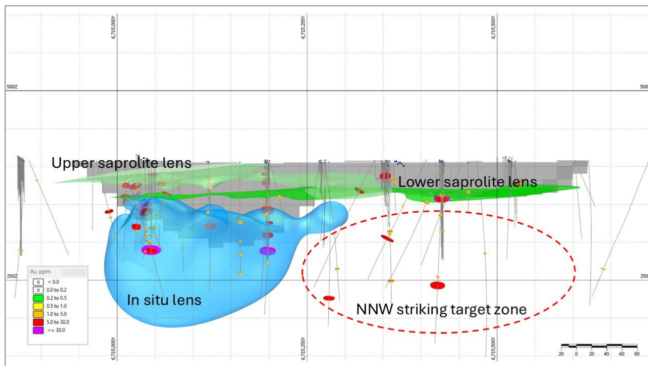
Figure 3: Looking west, showing the Upper and Lower Saprolite and In situ lenses, the optimised pit shell and resource extension target zone in red.
