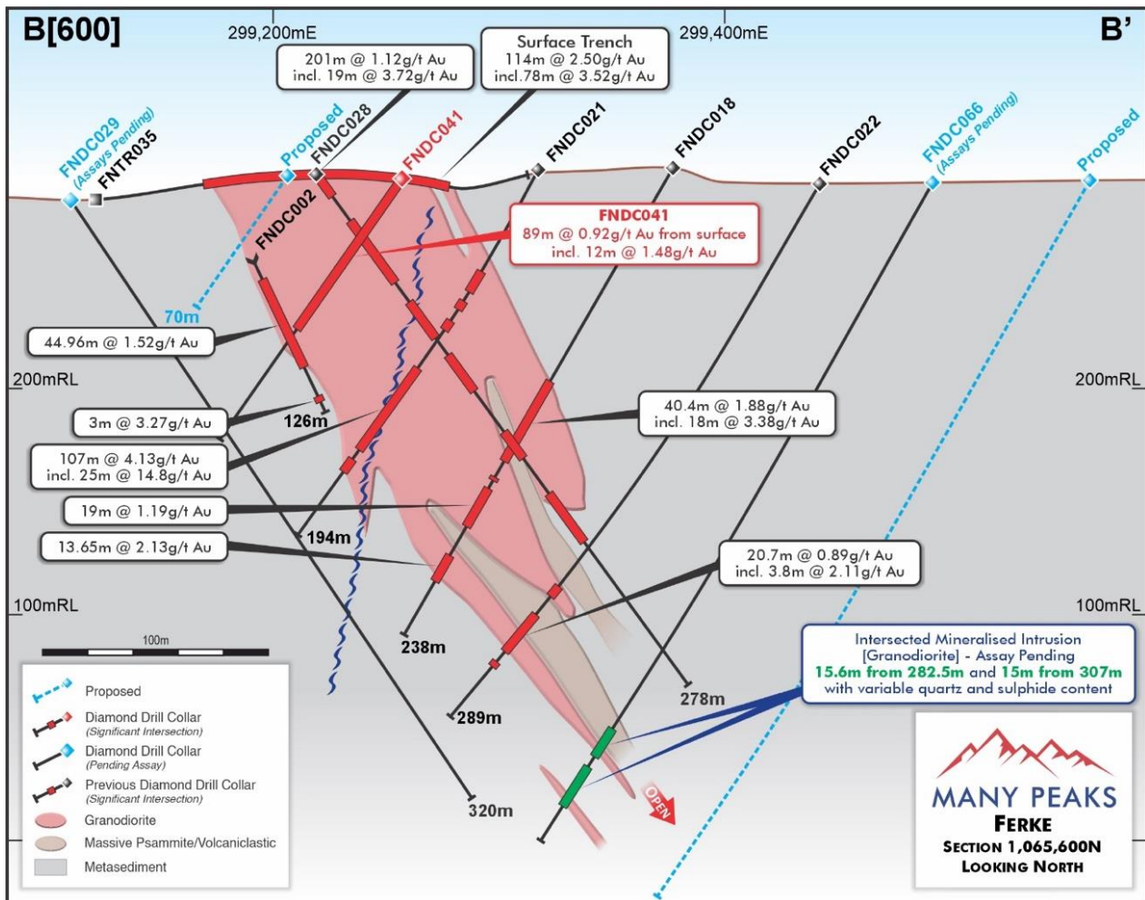
Figure 4 | Cross Section 1,065,450N with interpreted geometry of intrusions and location of significant intercepts in drilling
