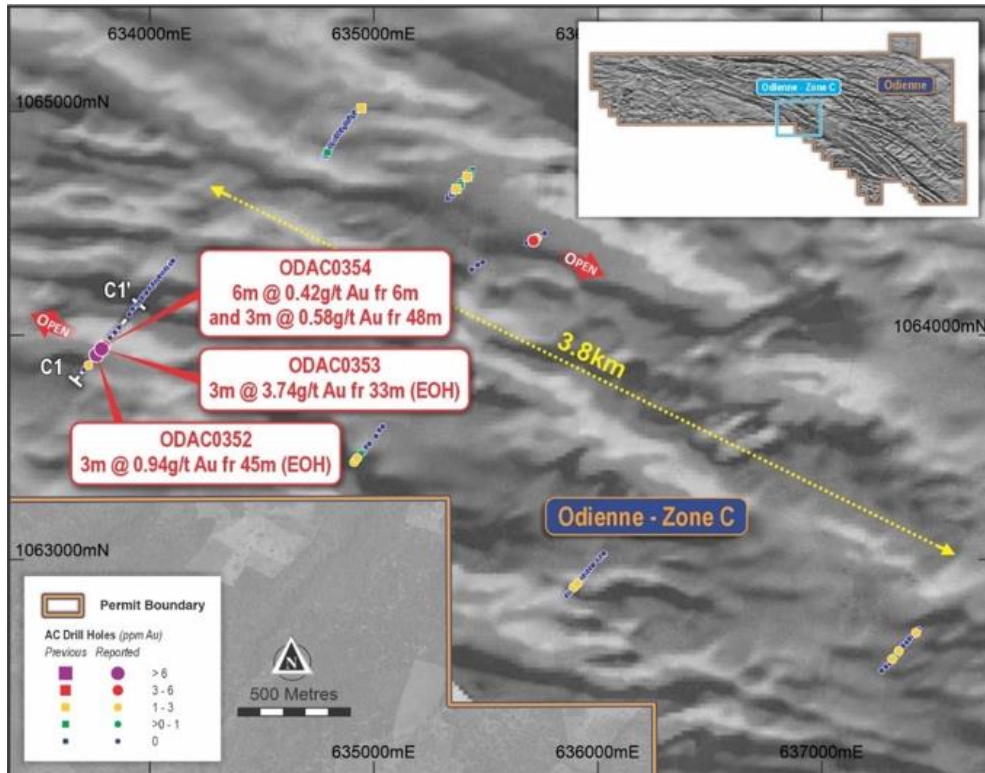
Figure 9 | Zone C Prospect area with AC collar locations projected on airborne magnetic imagery
