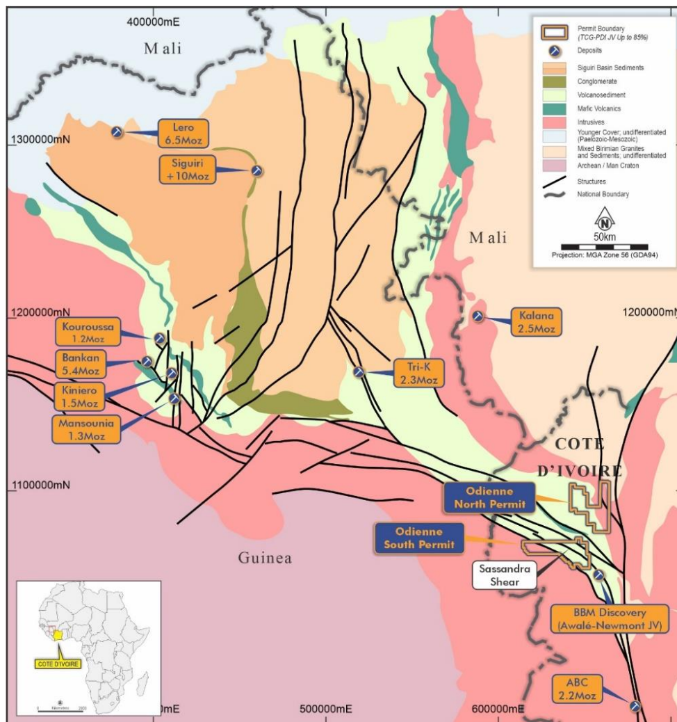
Figure 7 | Odienné Project location in the context of Siguiri Basin geology compilation and gold project locations regionally
