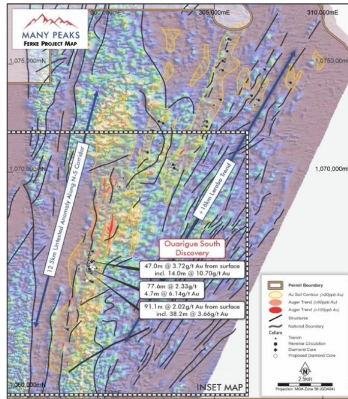
Figure 6 | Ferké Project area with location of previous soil, trench, RC and diamond locations in context of the reported auger target outlines.
