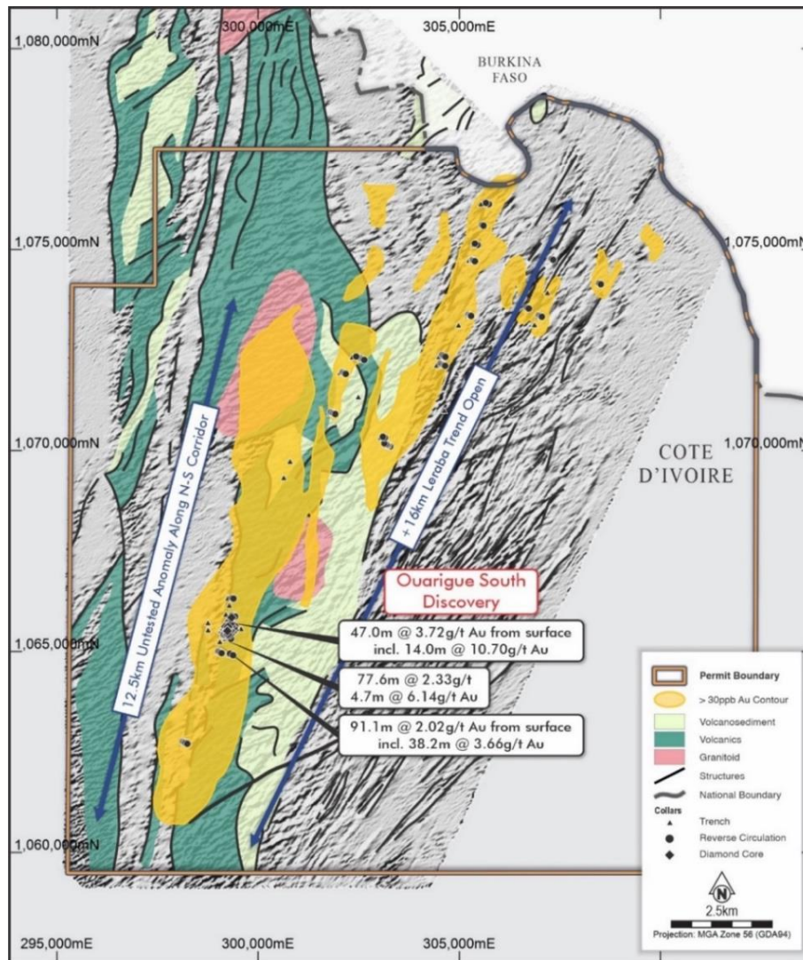
Figure 2 | Ferké Gold Project outline in relation to intersecting regional scale shear zones
