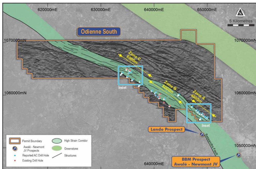
Figure 8 | Odienné Gold Project, Odienné South permit location with drill collar locations and locations of inset maps (Figure 9) over previously reported airborne magnetic imagery (1st derivative, Reduced to Pole processing)
