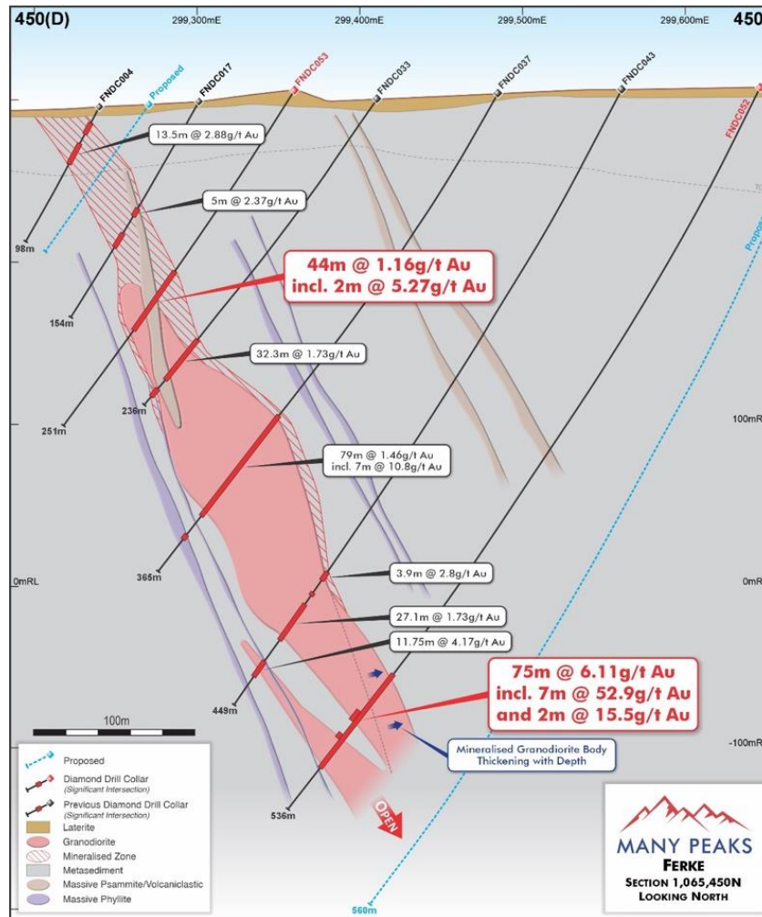
Figure 5 | Cross Section 1,065,450N with interpreted geometry of intrusions and location of significant intercepts in drilling
