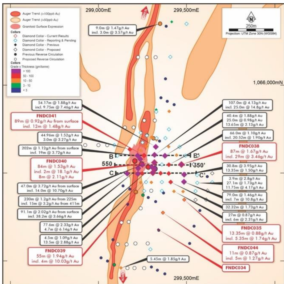
Figure 3 | Ouarigue Prospect within the Ferké project with assays results highlighted in red from the ASX announcement dated 15 July 2025.
