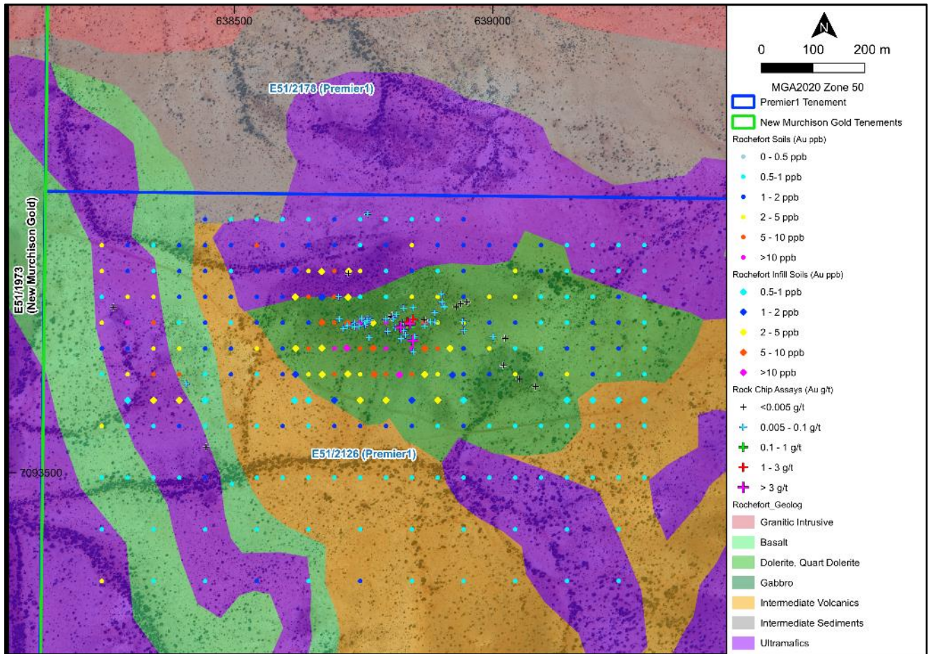
Figure 3: Abbotts North – Rochefort Prospect soil sampling program – Au ppb
