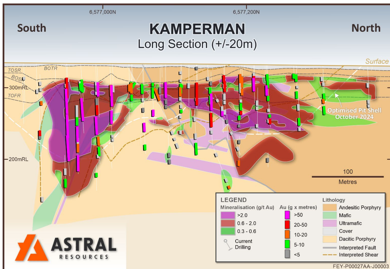
Figure 16 – Kamperman long section (Section 4) (see Figure 12 for section location).
