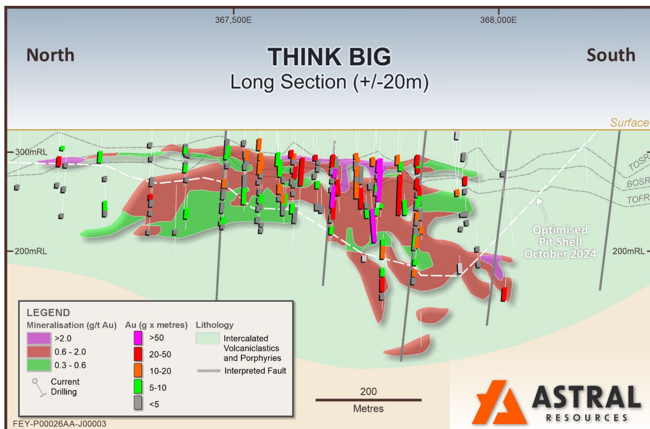
Figure 14 – Long section (Section 2) at Think Big illustrating interpreted mineralisation (refer to Figure 12 for section location).
