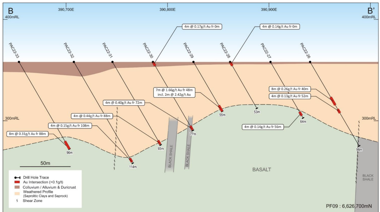
Figure 13. PF09 Prospect Section 6,626,700mN
