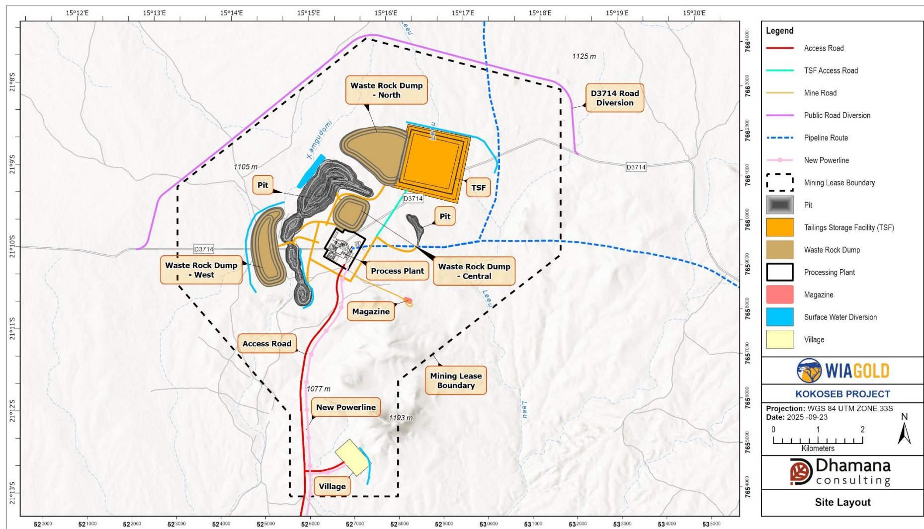
Figure 5 – Site Layout
