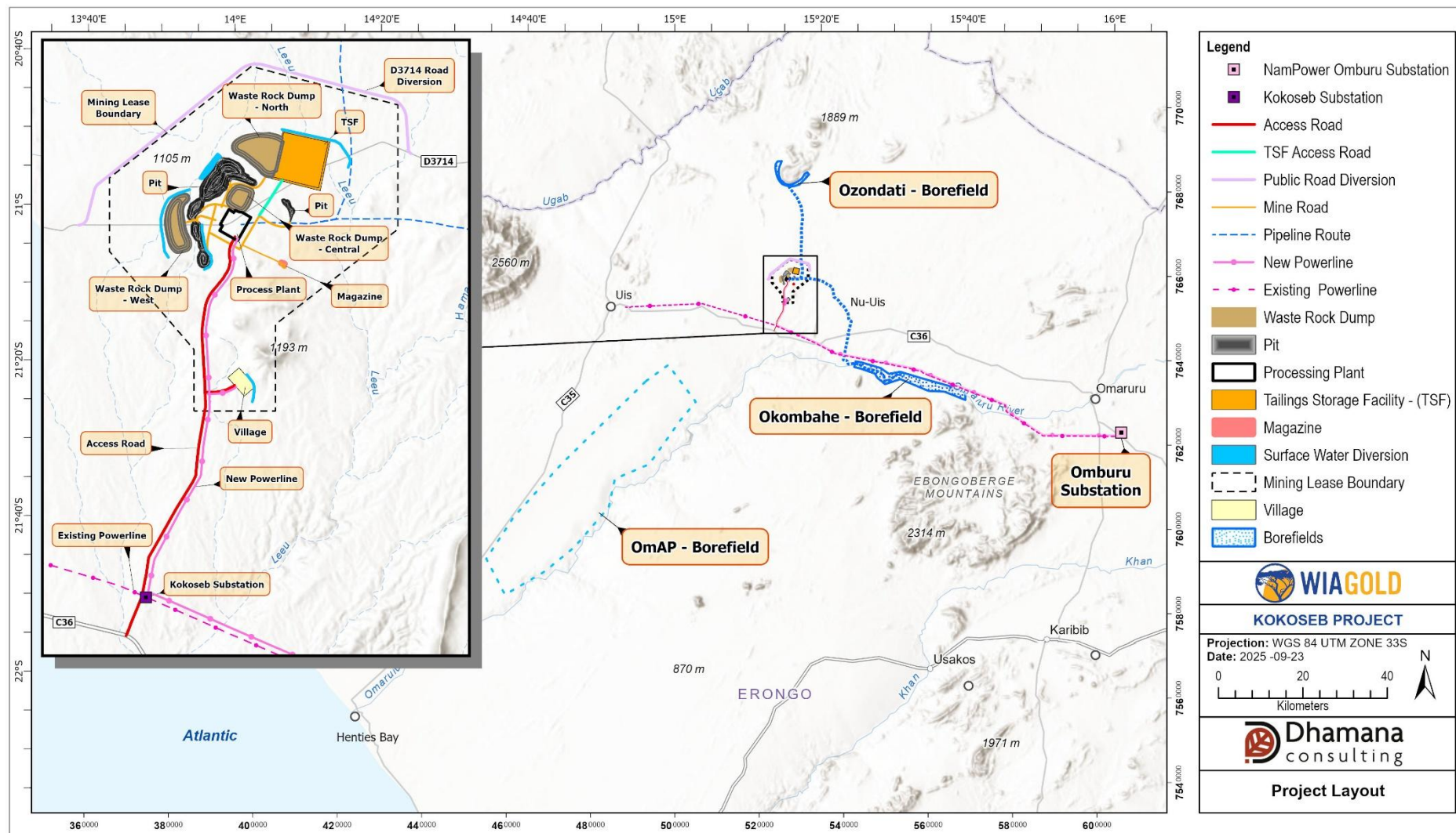
Figure 4 – Project Layout
