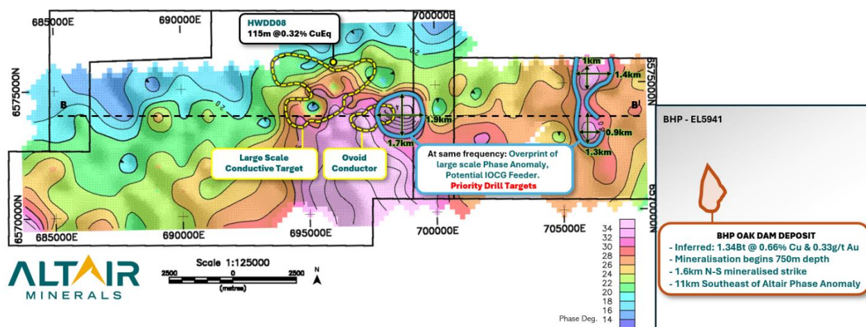
Figure 1: Forward AMT Model Plan View for Phase Anomalies at 4.06Hz frequency, with two major conductive targets. Model generated by Adelaide Mining Geophysics Pty Ltd - Jim Hanneson 3456
