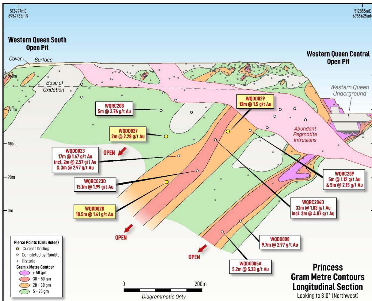
Figure 5 - Princess gram x metre contours with selected drill hole intersections – Longitudinal Section
