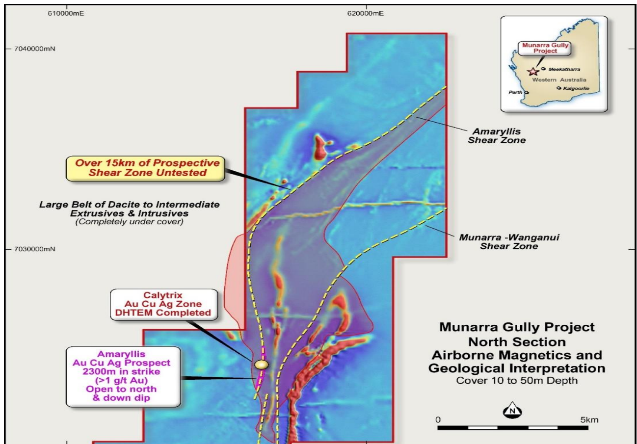
Figure 13 - Munarra Gully Project – Calytrix Location and Results over Airborne Magnetics
