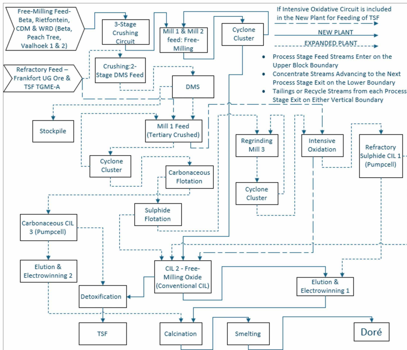
Figure17: Process Flow Schematic by Minxcon Showing both the New and Expanded Plant
