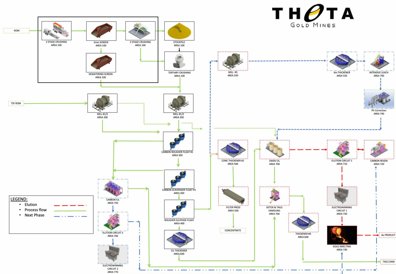
Figure 16: Process Flow Schematic by RM Process Showing both the New and Expanded Plant
