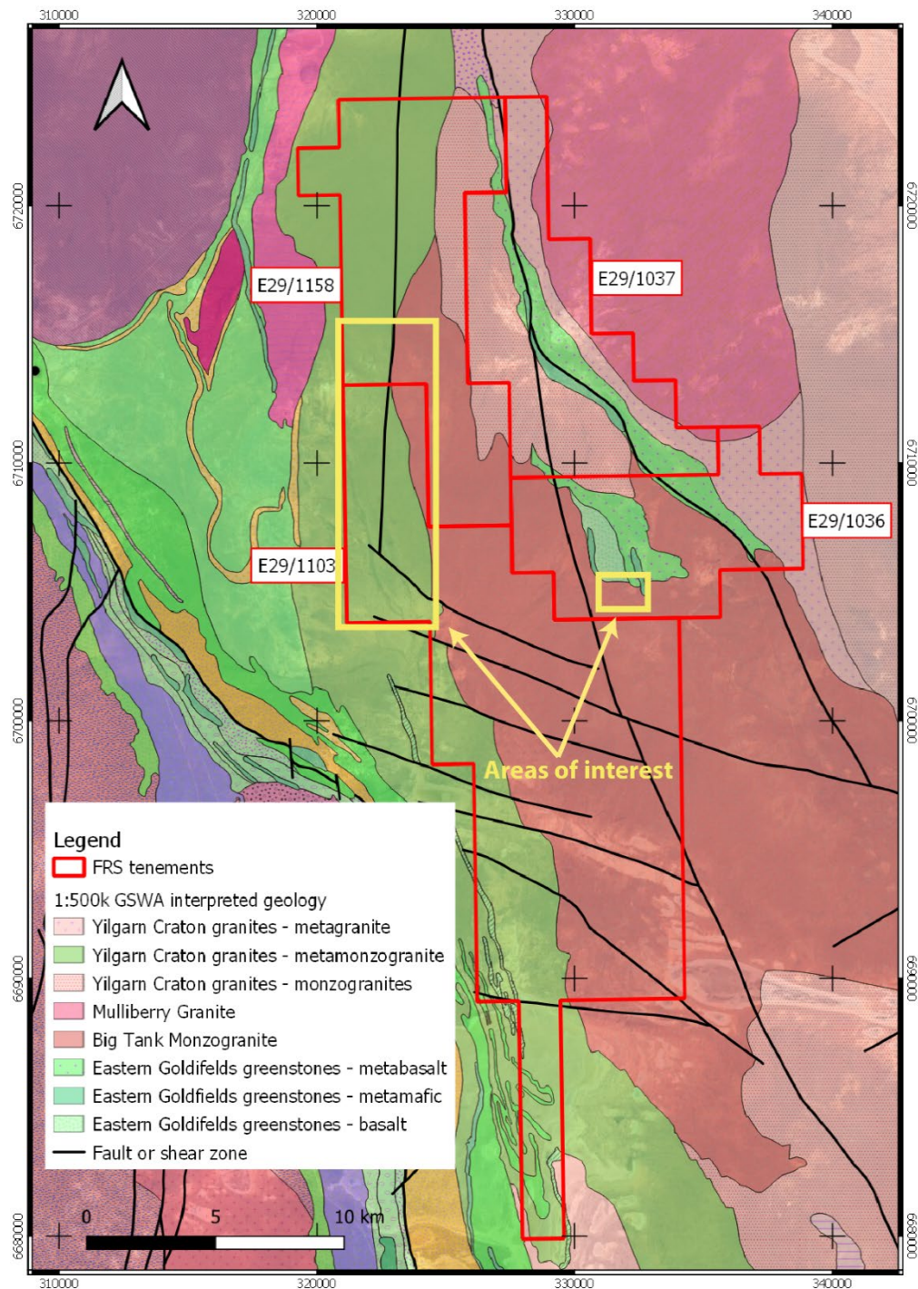
Figure 32. GSWA lithology
