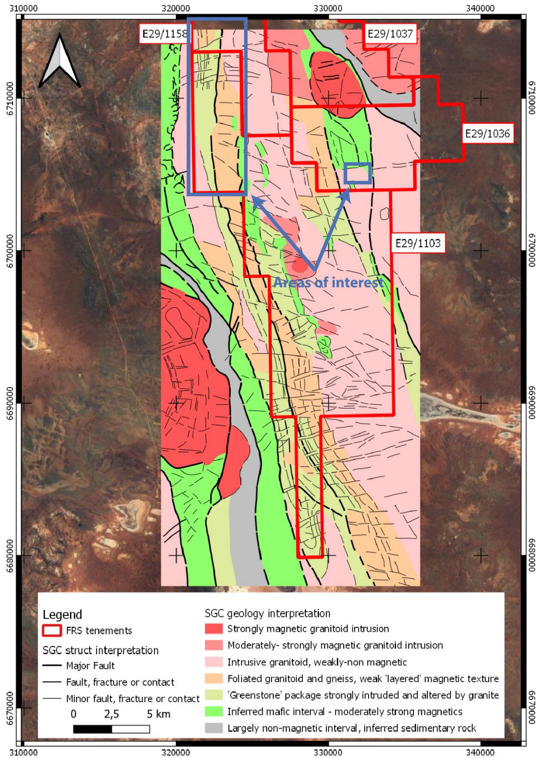
Figure 33. SGC interpreted lithology
