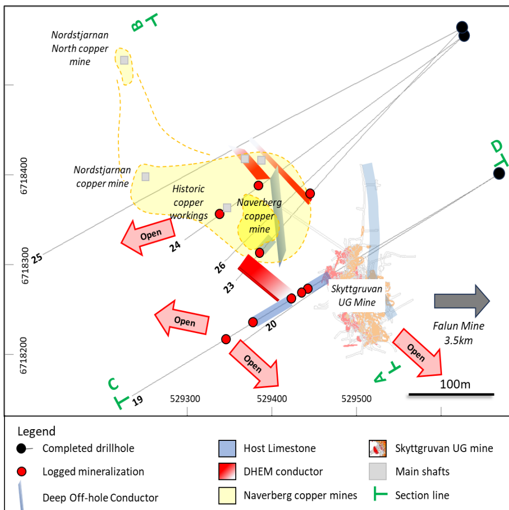
Figure 2: Plan view of completed drilling at Skyttgruvan-Naverberg
