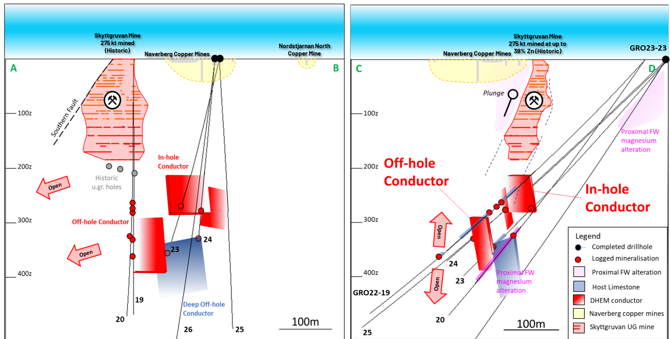
Figure 3: Long section and cross section of completed drilling at Skyttgruvan-Naverberg 1,5,6
