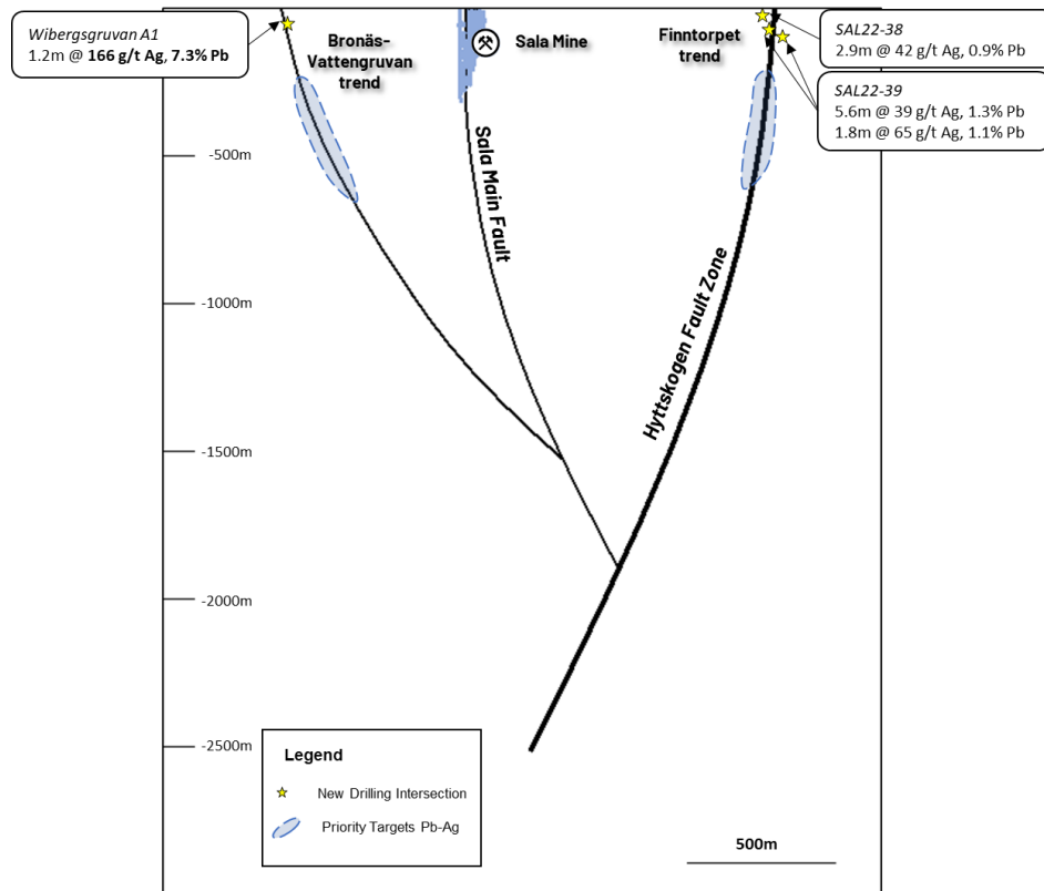
Figure 5: Simplified exploration model targeting high-grade galena-silver mineralisation. 8 Long section looking towards the east.
