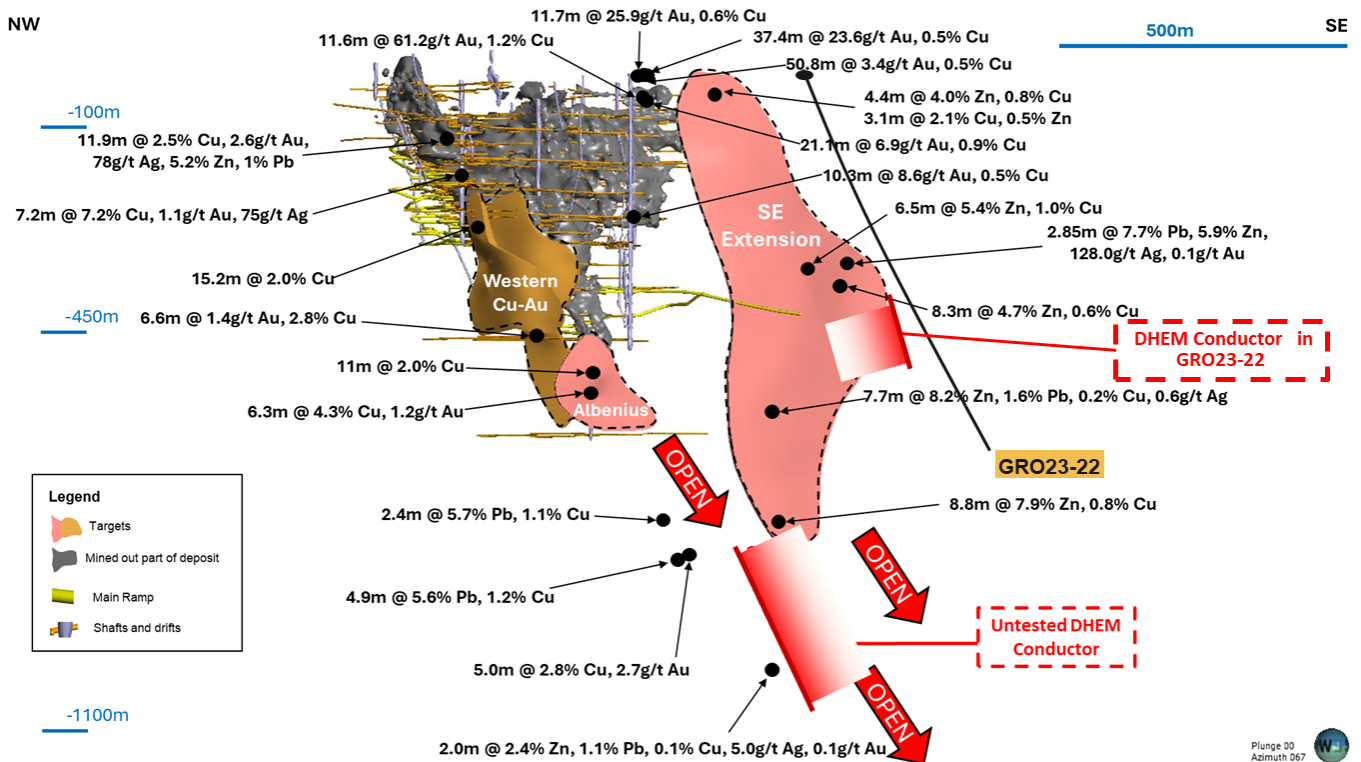
Figure 4: Long section of Falun, including hole GRO23-22 from recent Phase 1 drill program 1,2,6,7
