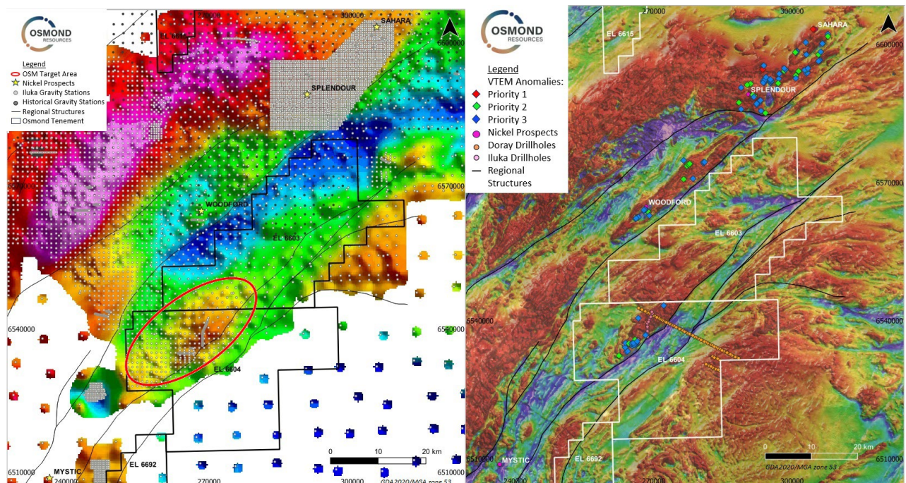
Figure 3: Fowler Project, a) existing gravity dataset with main target area for upcoming detailed gravity survey, b) VTEM anomalies identified by Iluka 2015 VTEM survey on detailed Total Magnetic Intensity image
