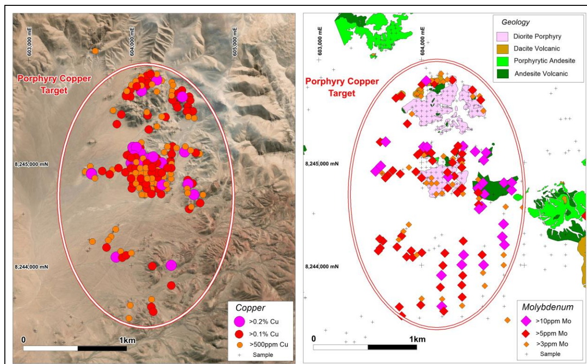
Figure 1: Cangallo Porphyry Copper Prospect showing anomalous copper and molybdenum values.
