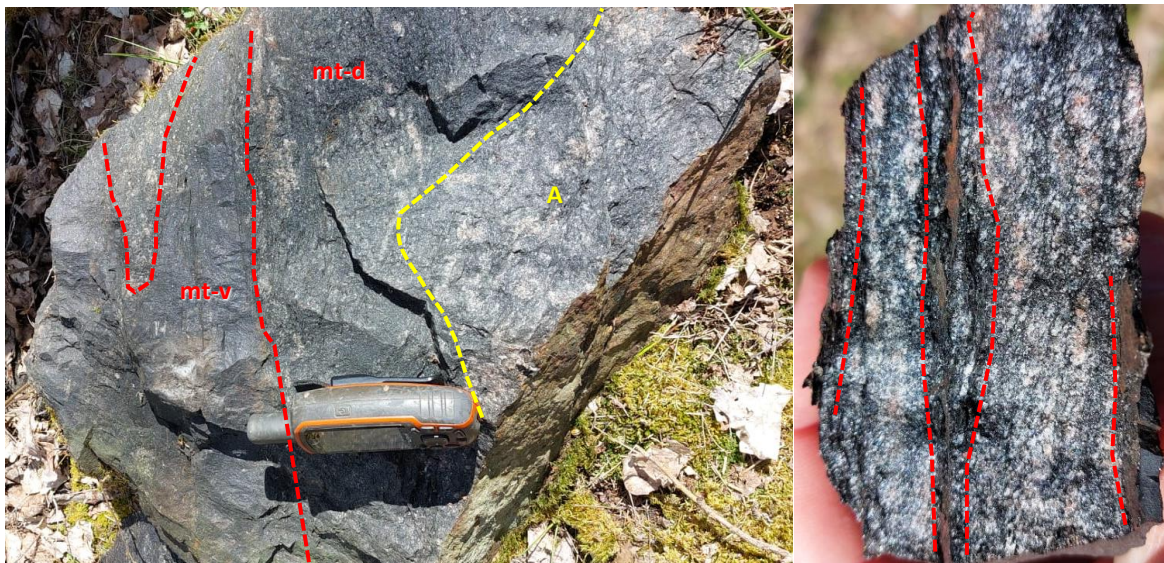
Figure 2A (left): Photograph of rock sample OLSGS003 with massive magnetite veins (mt-v) that returned 8,286 ppm TREO (86% HREO) as well as disseminated magnetite-altered (mt-d) augen gneiss (A).
