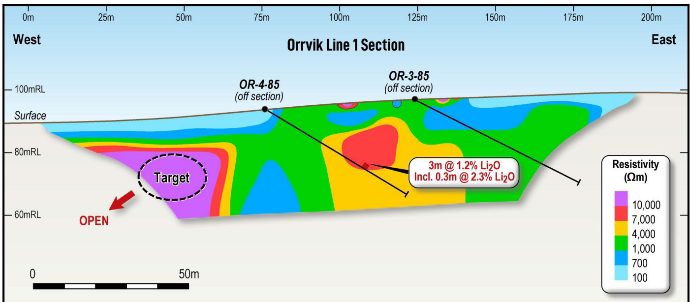
Figure 4: Orrvik Section Line 1. Inverted resistivity model section showing a strong resistive body that appears to be disjointed from Lines 2 and 3 possibly indicated a change in geology possibly related to faulting. Historical drill hole OR-4-85 intersected 3m at 1.2% \text{Li}_2\text{O} associated with a strong resistive anomaly. A large stronger anomaly to the west has not been drill tested.
