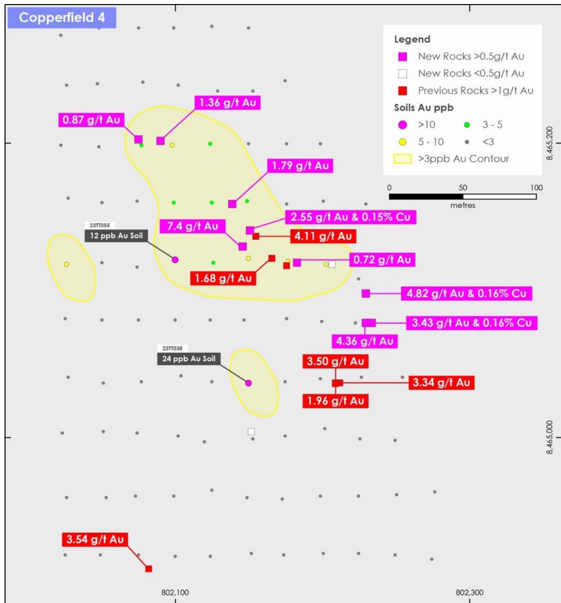
Figure 3 – Copperfield 4 prospect with current and historical rockchip and soil samples.
