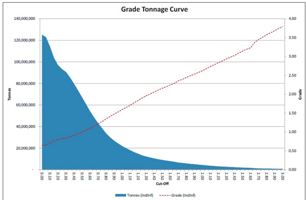
Figure 2.9: Kobada grade-tonnage curve for Mineral Resources
