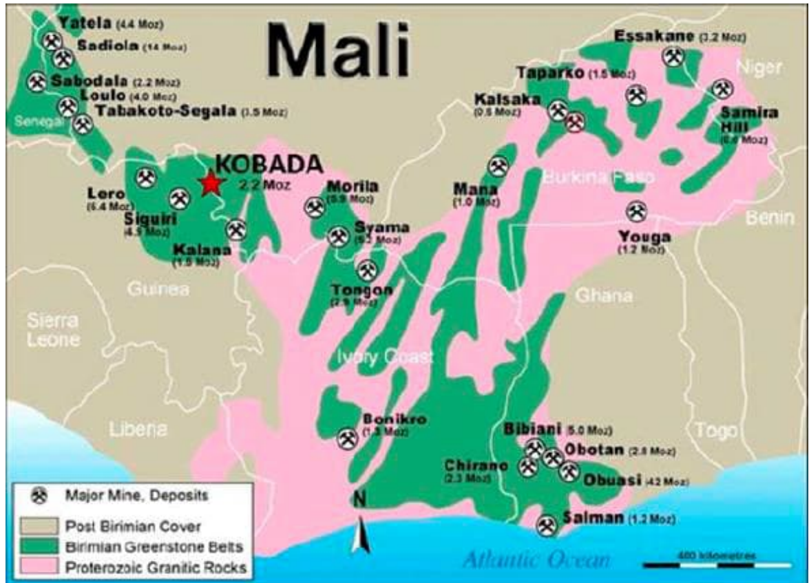
Figure 2.4: Greenstone belts and major gold mines of Regional West Africa
