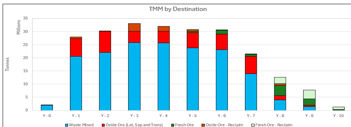
Figure 2.16: Mining strategic schedule by material type
