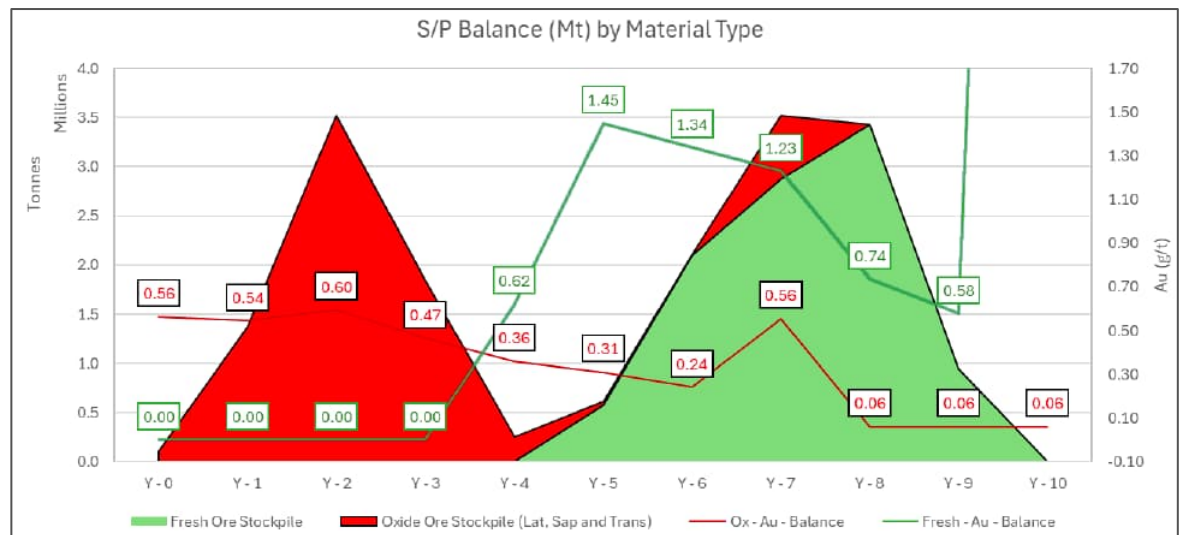
Figure 2.15: Stockpile balance and grade by material type
