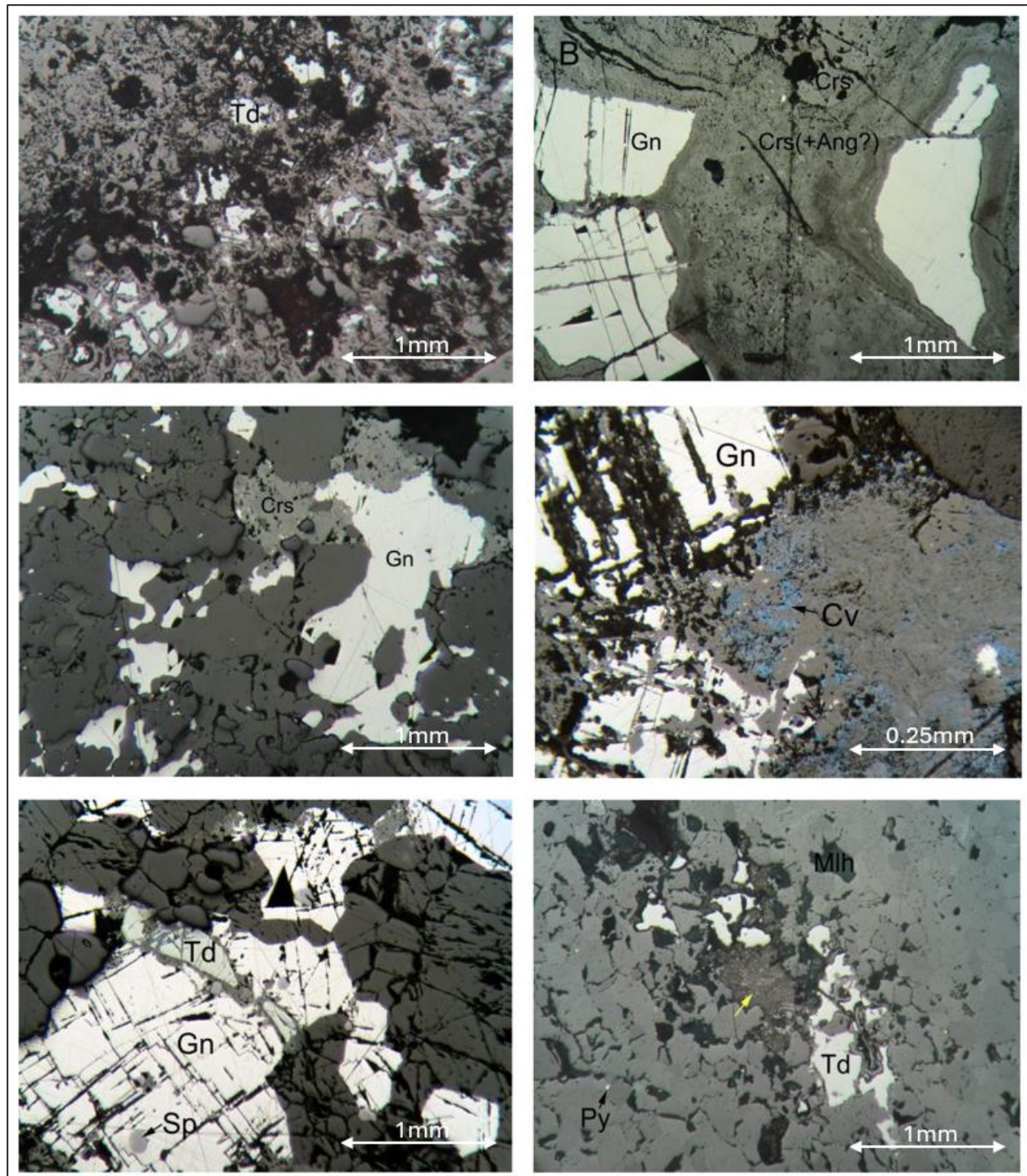
Figure 9: Kovacevac Prospect (location of sample SIRC472, refer Figure 6), microphotographs of polymetallic mineralogy; minerals: Td – tetrahedrite, Gn – galena, Crs – cerussite, Ang – anglesite, Cv – covellite, Sp – sphalerite, Py – pyrite.
