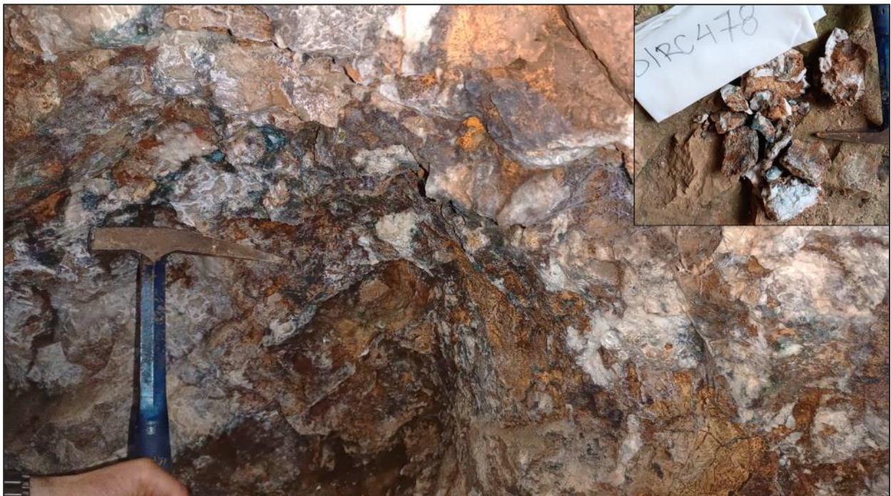
Figure 8: Kovacevac Prospect (west part), secondary iron oxides and hydroxides in limestone surrounding barite-quartz veining with malachite-azurite staining
