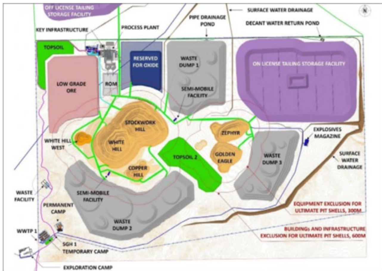
Figure 4-4: Kharmagtai proposed site layout.
