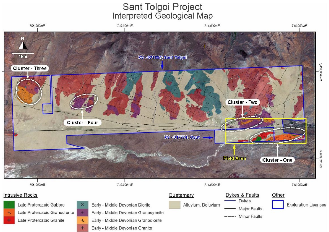
Figure 3-8: Interpreted geology of Sant Tolgoi project area.
