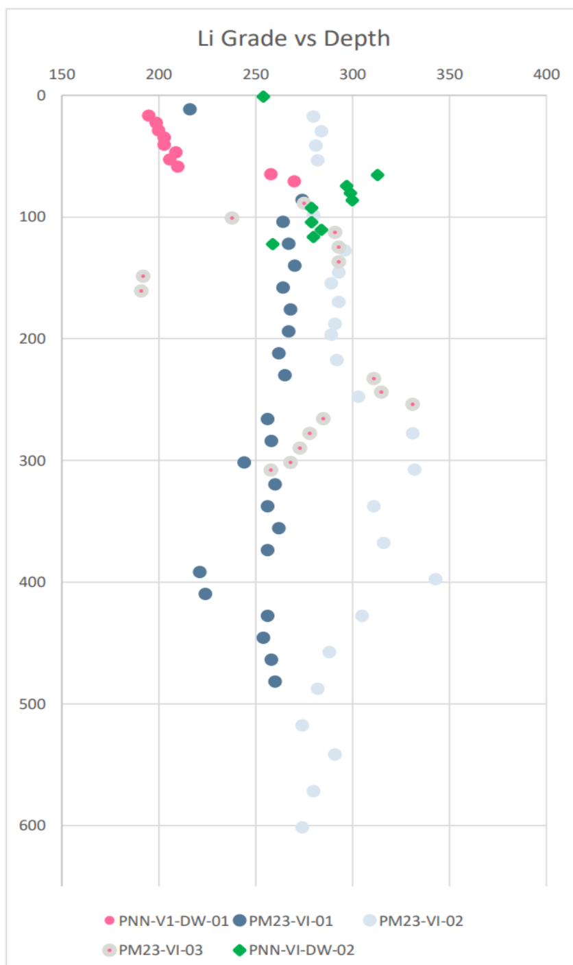
Figure 2: Lithium grades in each drillhole plotted as grade vs depth.
