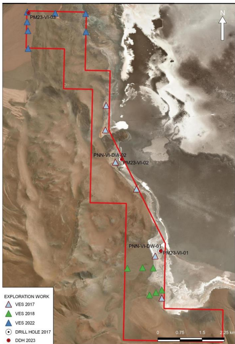
Figure 1: Location plan of Power's lithium brine resource drilling and exploration, Rincon salar. (VES: Vertical Electrical Sounding geophysical survey).
