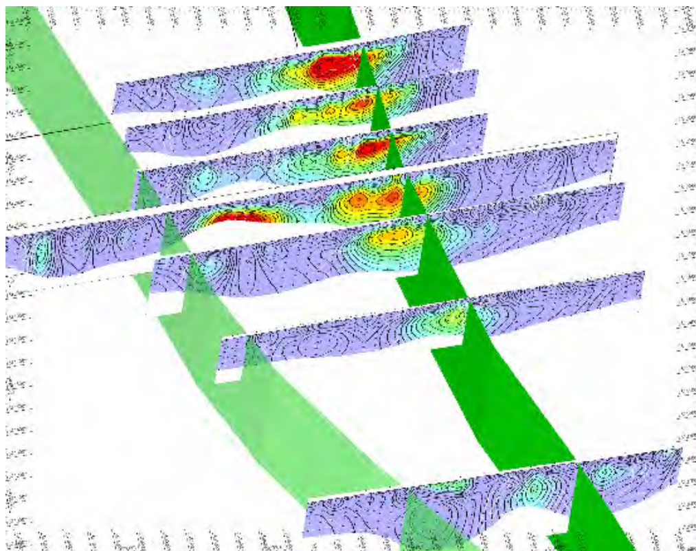
Figure 2: Stacked I.P. survey lines and chargeability between regional faults at Mogul VMS project.
