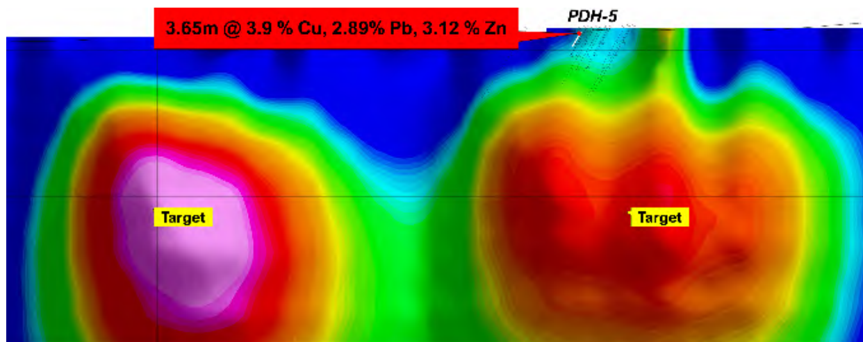
Figure 4: Western and Eastern I.P. targets from 2023 IP Survey on Line 7,572,100mN.
