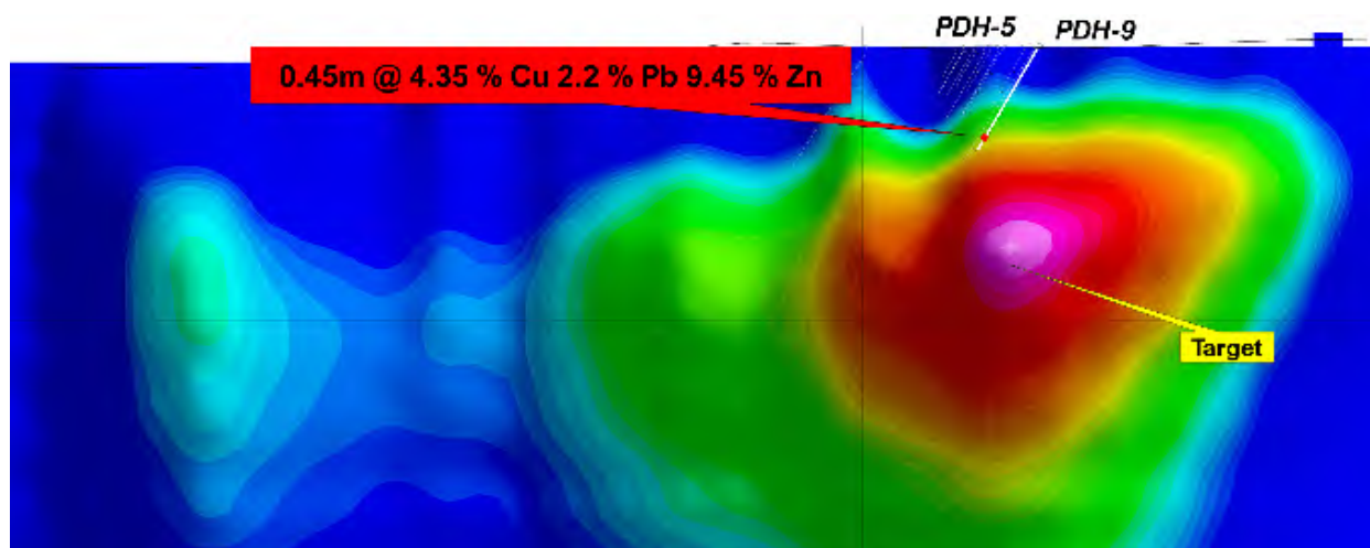
Figure 3: Eastern I.P. target from 2023 IP Survey on Line 7,572,300mN down dip from high-grade, near surface mineralisation.
