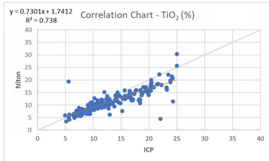
Figure 6-8 – Resampling program comparative analysis plots for \text{TiO}_2 – Portable XRF Versus ICP: Correlation Chart
