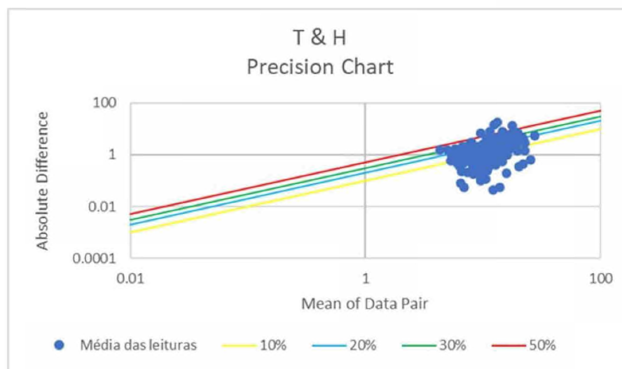
Figure 6-10 – Resampling program comparative analysis Precision Chart plots for TiO 2 – Portable XRF Versus ICP
