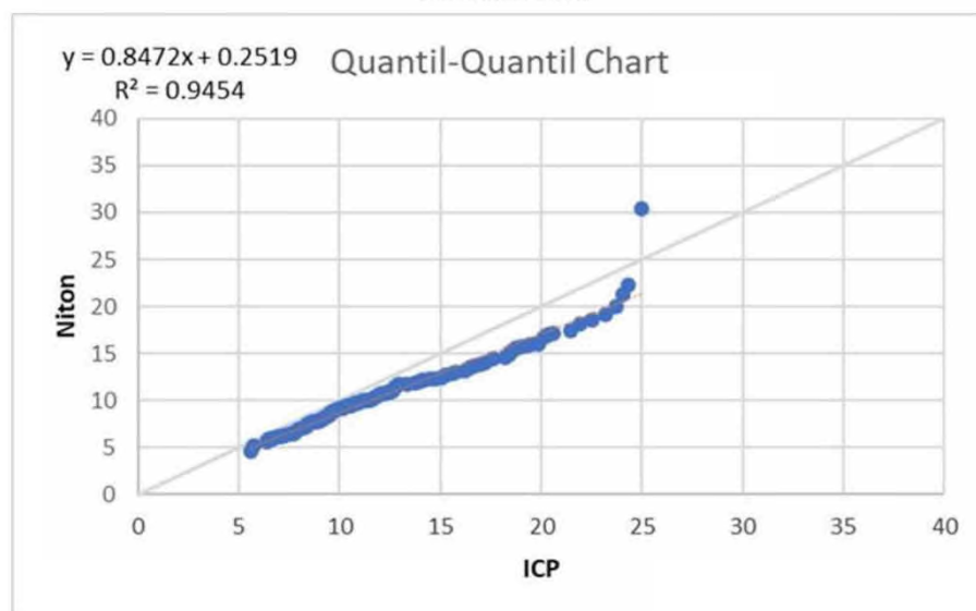
Figure 6-9 – Resampling program comparative analysis plots for \text{TiO}_2 – Portable XRF Versus ICP: Quantil-Quantil
