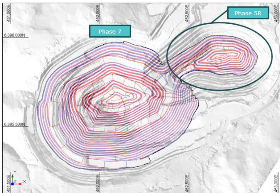
Figure 5.6 Plan view of the Main Zone and East Zone pits
