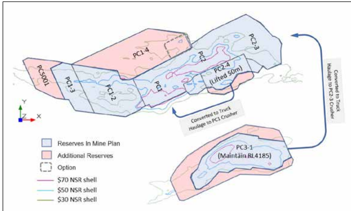
Figure 2.13 Cadia East panels
