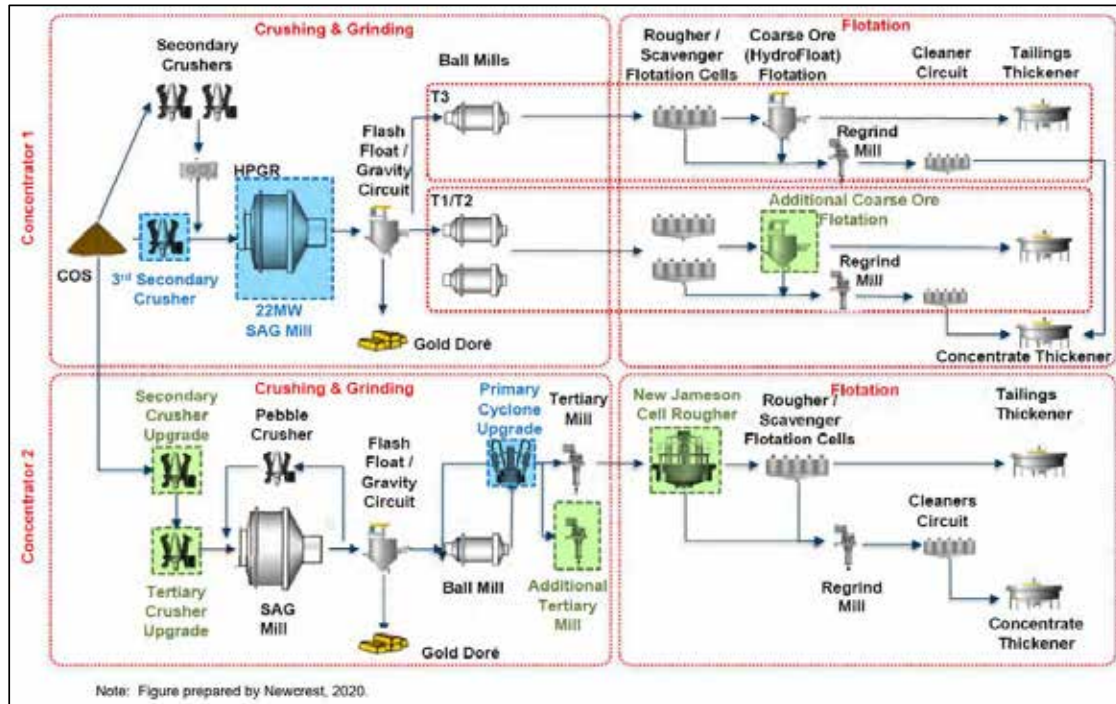
Figure 2.14 Simplified process flow sheet for Concentrator 1 &amp; 2
