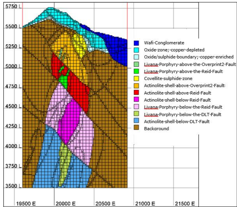
Figure 7.7 Copper estimation domains
