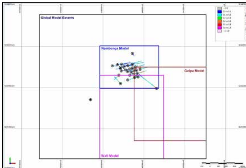
Figure 7.12 Nambonga drillhole traces.
