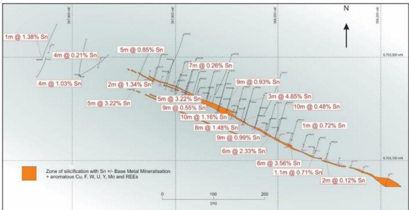
Figure 6: Plan of South Ridge drilling with significant historical drill intersections
