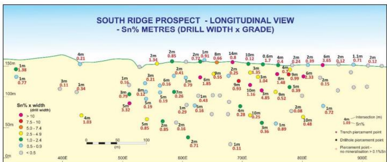
Figure 7: Long Section of South Ridge Prospect with grade x width intersections shown
