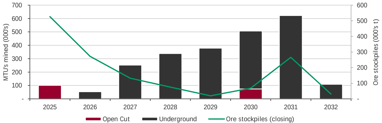
Figure 9.4: MTUs mined
