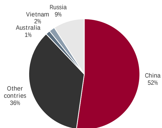
Figure 7.2: Global Reserves 2023
