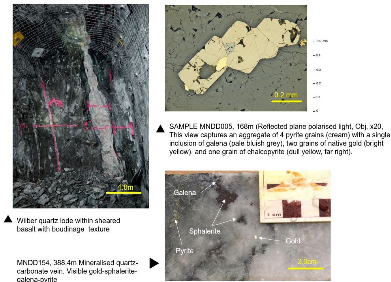
Figure 9 – Mineralisation at Andy Well.
