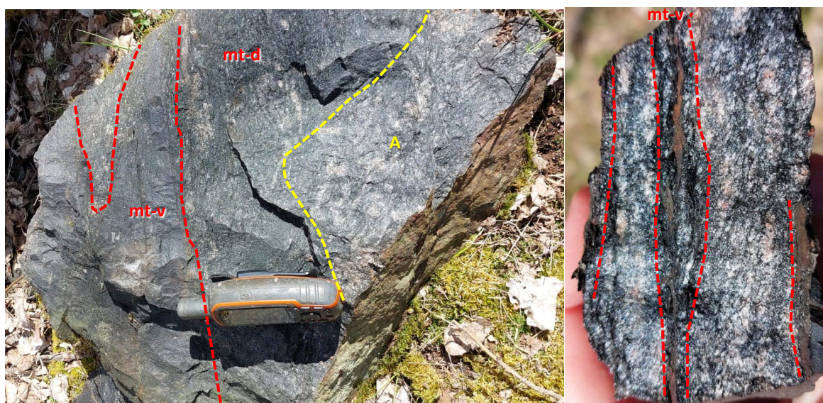
Figure 1A (left): Photograph of rock sample OLSGS003 with massive magnetite veins (mt-v) that returned 8,286 ppm TREO (86% HREE) as well as disseminated magnetite-altered (mt-d) augen gneiss (A). Figure 1B (right): Photograph of rock sample OLSGS001 of biotite-altered augen gneiss with magnetite (mt) veins that returned 9,012 ppm TREO
