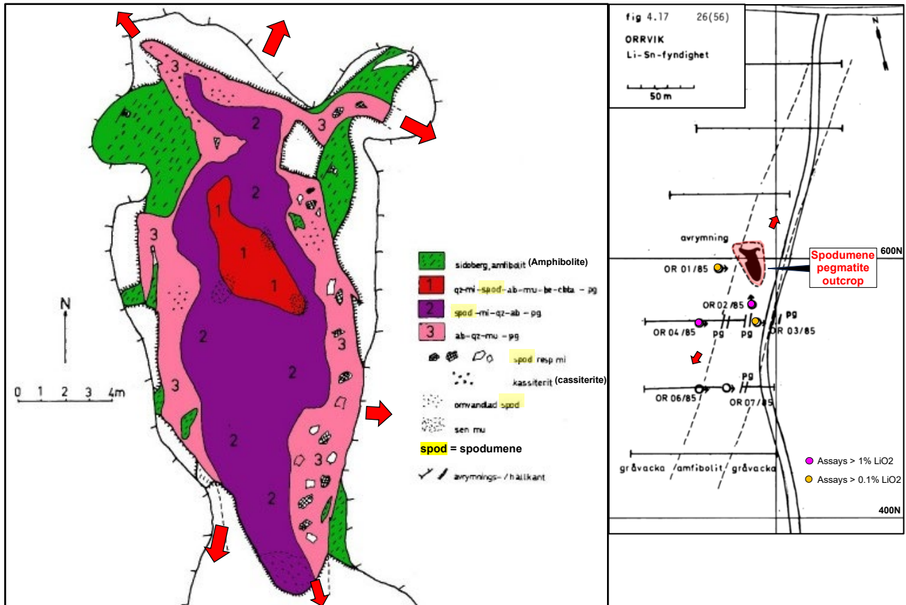
Figure 3A (left): Mapping of the exposed spodumene-bearing pegmatite at Orrvik by LKAB in 1985. Red arrows indicate where the Orrvik pegmatite is open undercover. Spodumene mineralisation (spod) clearly marked in yellow. Figure 3B (right): Drill plan by LKAB in 1985 showing the location of the drill collars in relation to the spodumene pegmatite outcrop and amphibolite host rock. Red arrows indicate where mineralisation is still open.
