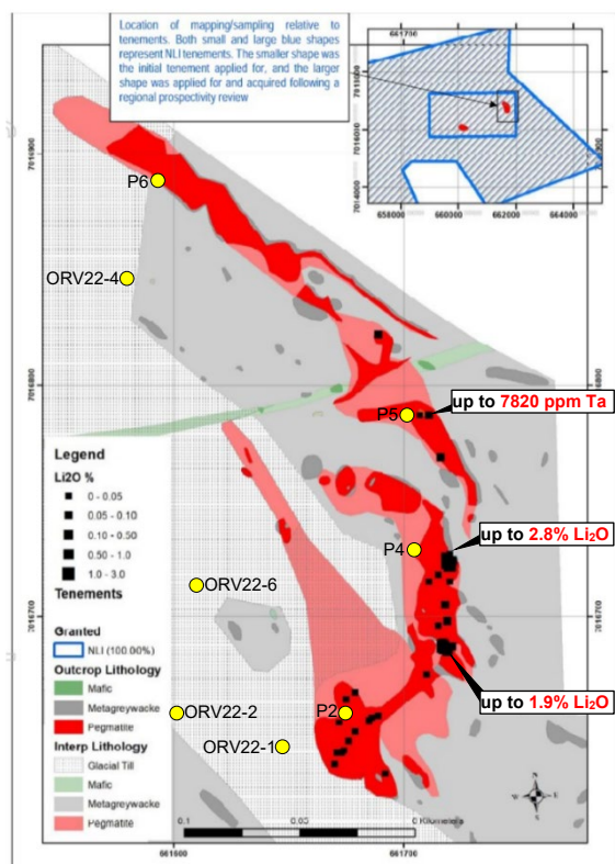
Figure 4 (left): Mapping by Novo Litio in 2017 showing the exposed Stenback LCT pegmatite and highlight results.
