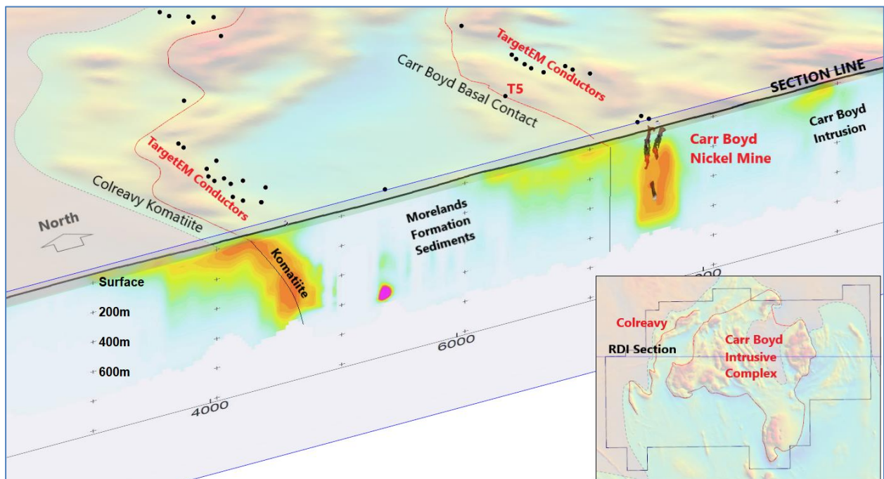
Figure 1: RDI slice through 6672920 North showing the Colreavy Komatiite and Carr Boyd Pyroxenite as interpreted from the AFMAG data along with bedrock conductors identified from the TargetEM system
