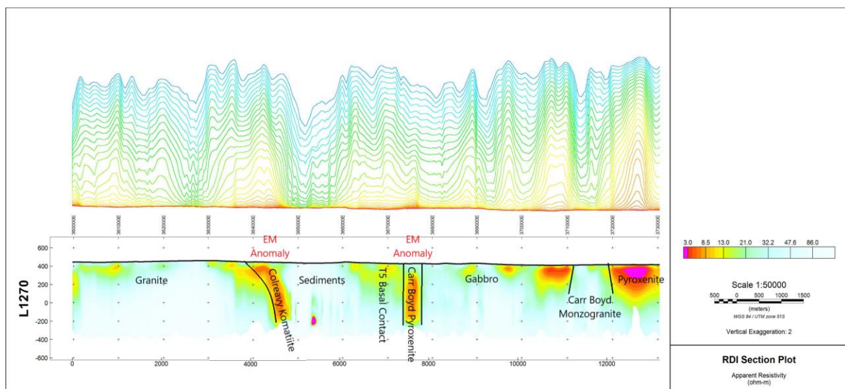
Figure 2: RDI slice through 6672920 North showing the Colreavy Komatiite and Carr Boyd Pyroxenite
