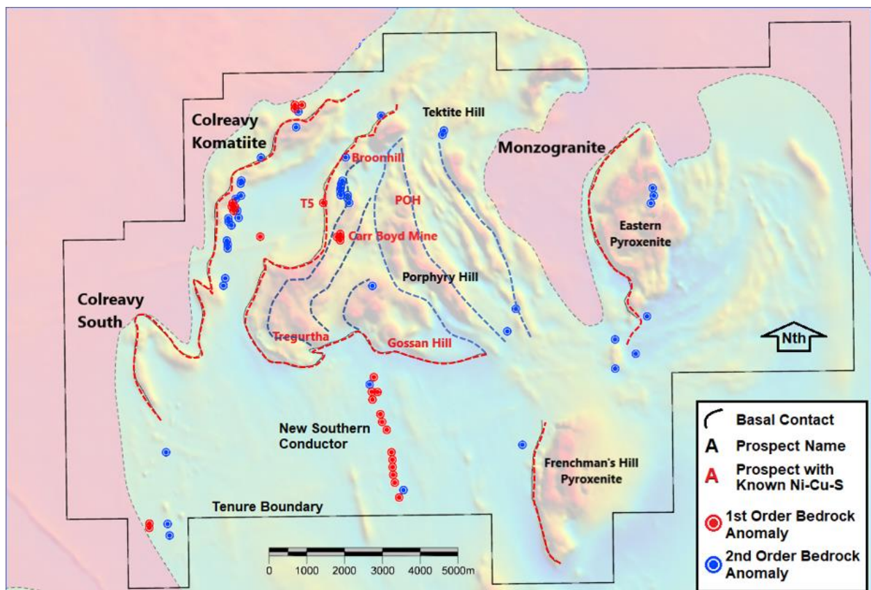
Figure 3: Correlation between internal and external basal contacts and the bedrock anomalies identified by the recent TargetEM survey
