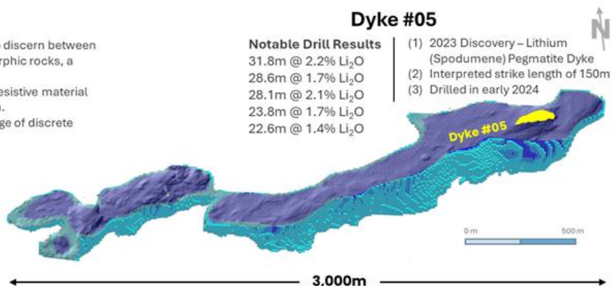
Figure 1: Trieste Lithium Project: Mobile MTm 3D model illustrating the three-metasediment hosted resistive trends.
