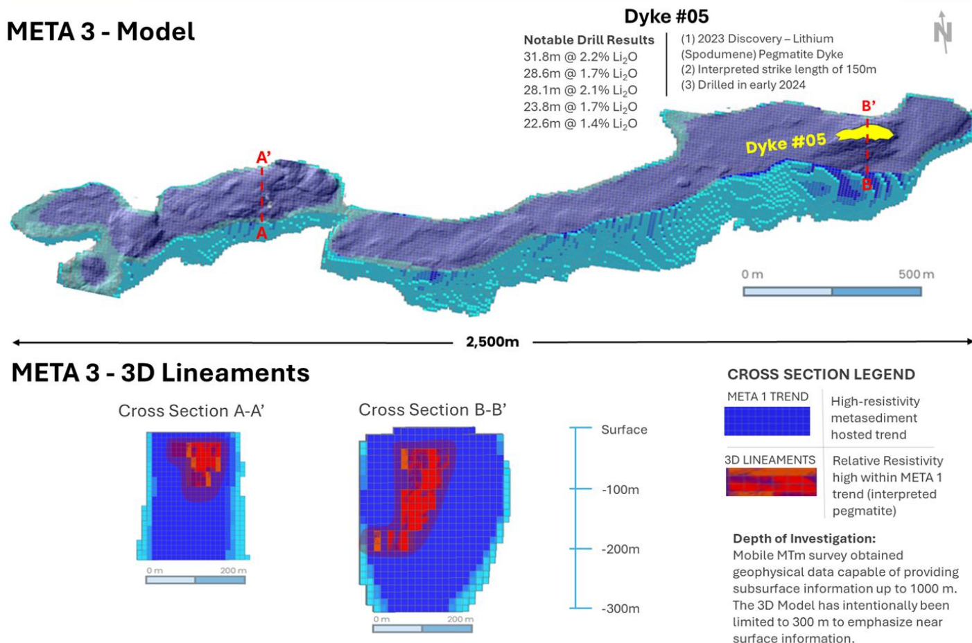
Figure 5: Trieste Lithium Project: META 3 Trend from Mobile MTm 3D model with superimposed 3D Lineaments.
