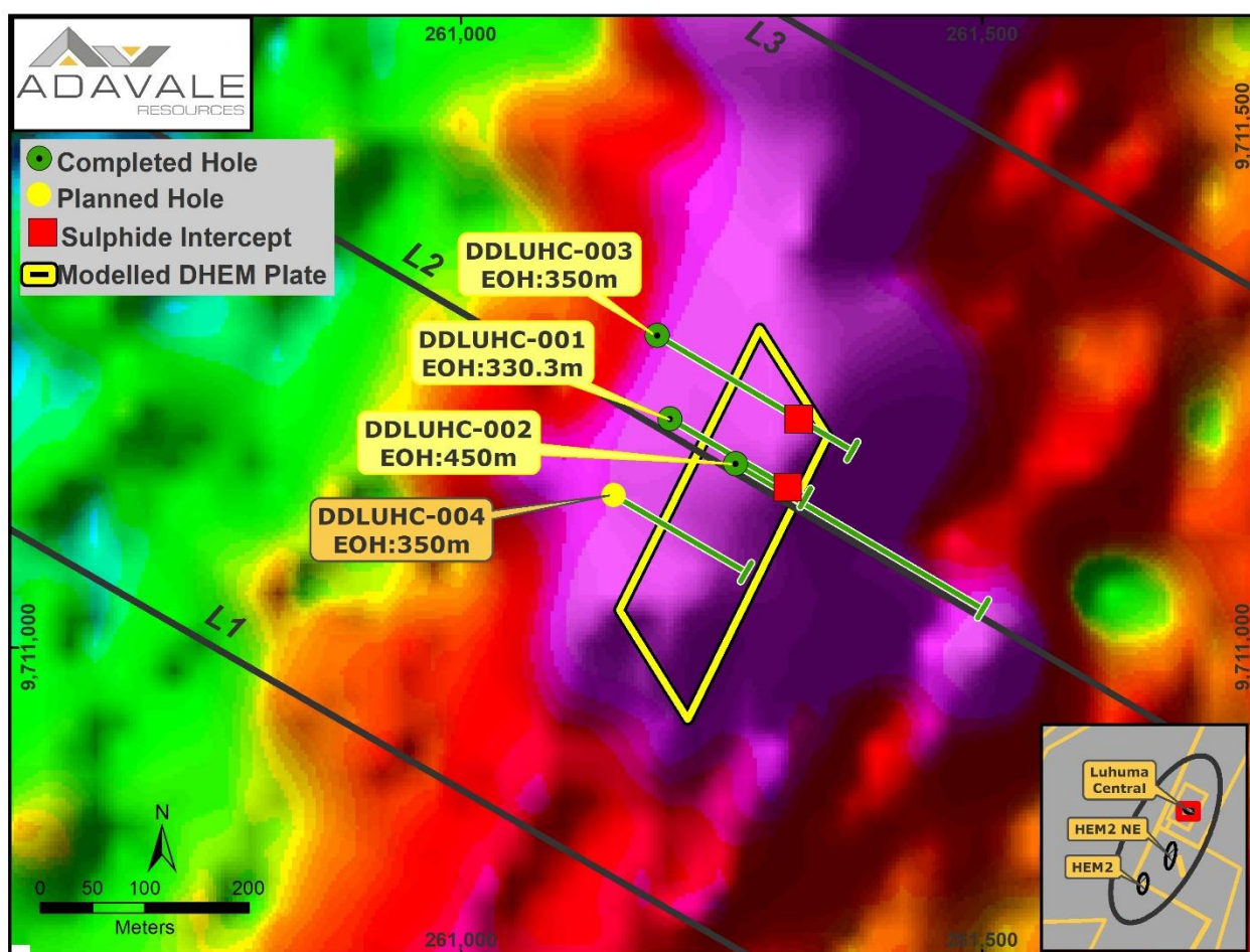
Figure 1: Drillhole traces targeting AMT anomaly and planned drillhole DDLUHC004 targeting the modelled DHEM plate. The red squares show where sulphides have been intercepted to date. Colour image background represents gridded C25 (db/dt) from the NRG Xcite airborne EM survey.
