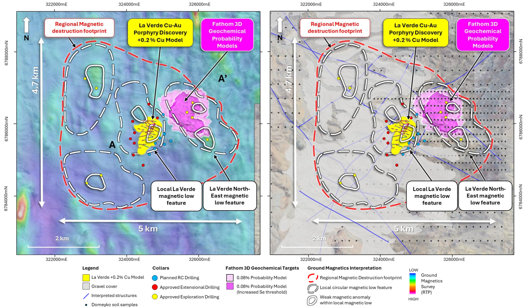
Figure 3. Plan view showing the La Verde +0.2% Cu mineralisation interpolant in relation to regional magnetic destruction footprint (red dashed), local magnetic low features (white dashed), weakly magnetic anomalies (white line) and Fathom 3D geochemical probability models (purple isosurfaces). Left – shown overlain on reduced-to-the-pole (RTP) ground magnetics. Right – shown in relation to mapped gravel cover, interpreted regional structures and soil sample coverage. See announcement dated 29 May 2025 for JORC Table 1 additional technical information.
