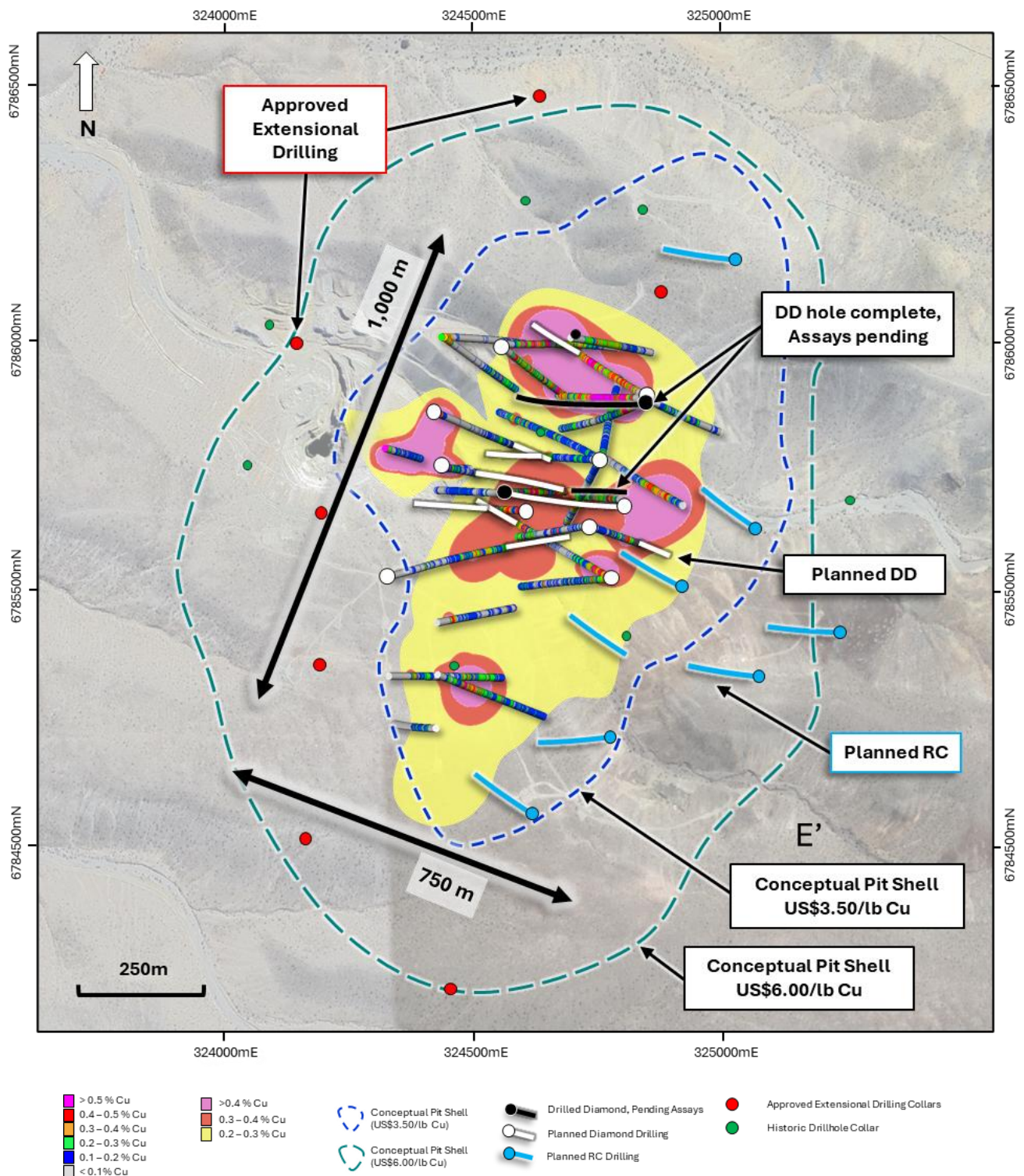
Figure 2. Plan view map of the La Verde porphyry system showing approved extensional collar locations (red points), planned (white traces) and completed DD drilling (black) compared with +0.2% copper (yellow), +0.3% copper (red), +0.4% copper (Magenta) mineralisation interpolants from Phase one drilling. Conceptual open pit shells 1 displayed for $US3.50/lb Cu (blue) and $US6.00/lb Cu (green) displayed as dashed lines. See announcement dated 25 September 2025 for JORC Table 1 additional technical information.
