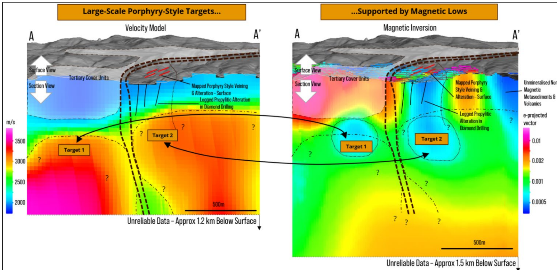
Figure 7 – Conceptual section and surface projection showing two porphyry targets at Scarlett based on velocity (left) and MVI (right) models. The circled areas in the MVI model represent regions where the high velocity targets coincide with lower magnetic response (ASX announcement dated 26 September 2024)
