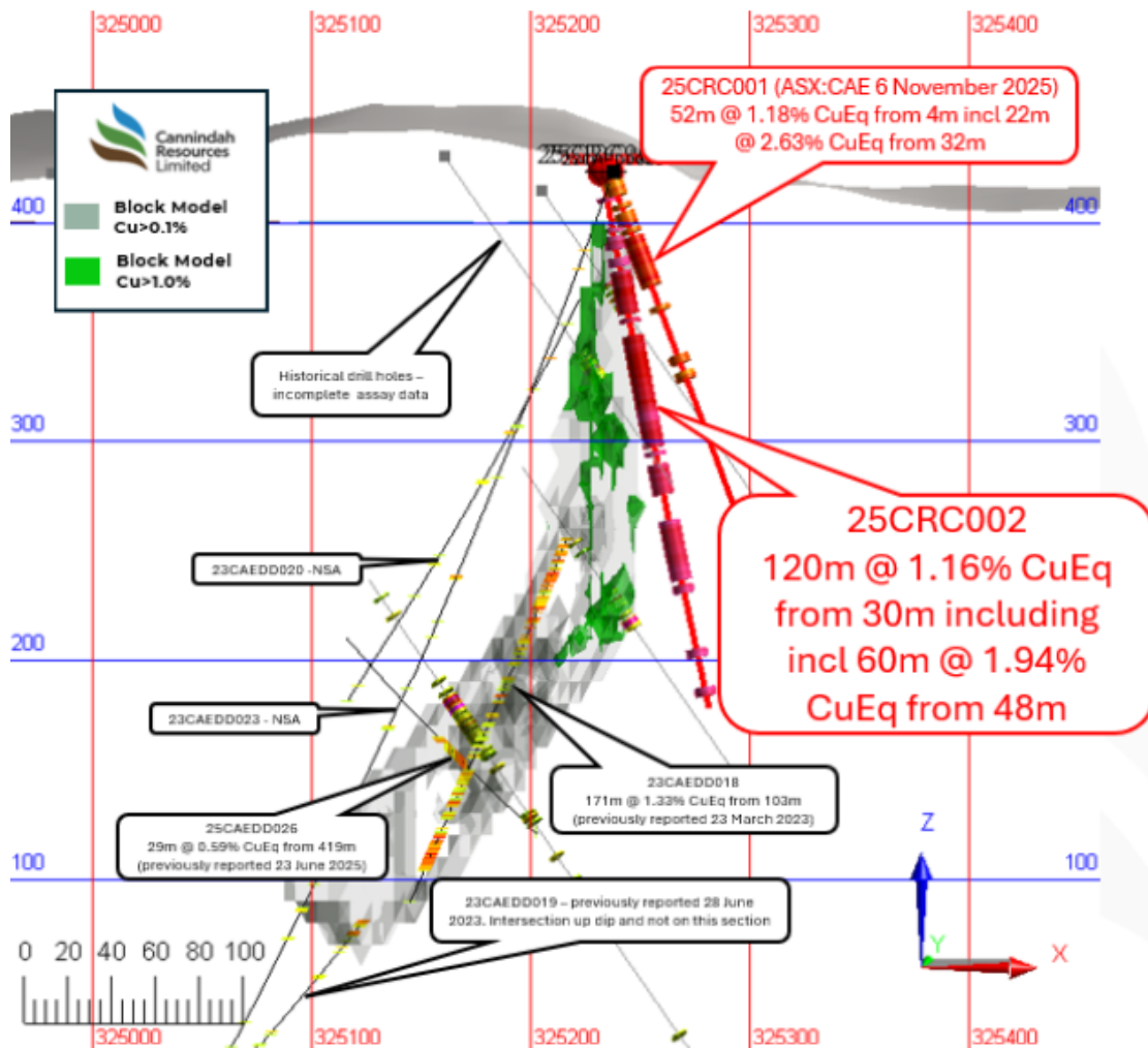
Figure 3: Cross section showing 25CRC001 and 25CRC002 in relation to previous historical drilling and block model. A plan of all drill holes is shown in Figure 2 . Downhole intersections are apparent and not true width.
