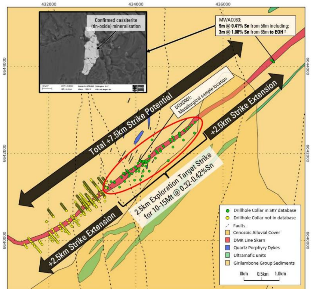
Figure 4: Plan showing the initial Exploration Target area and the extensions to potentially triple the Exploration Target along strike. Insert shows an image of the cassiterite (tin-oxide) (courtesy of UNSW) over 2.5km along strike beyond the margin of the initial Exploration Target and, to the southwest, the drillholes not currently in the SKY database. Showing that the Doradilla Tin Deposit continuous and open in all directions.
