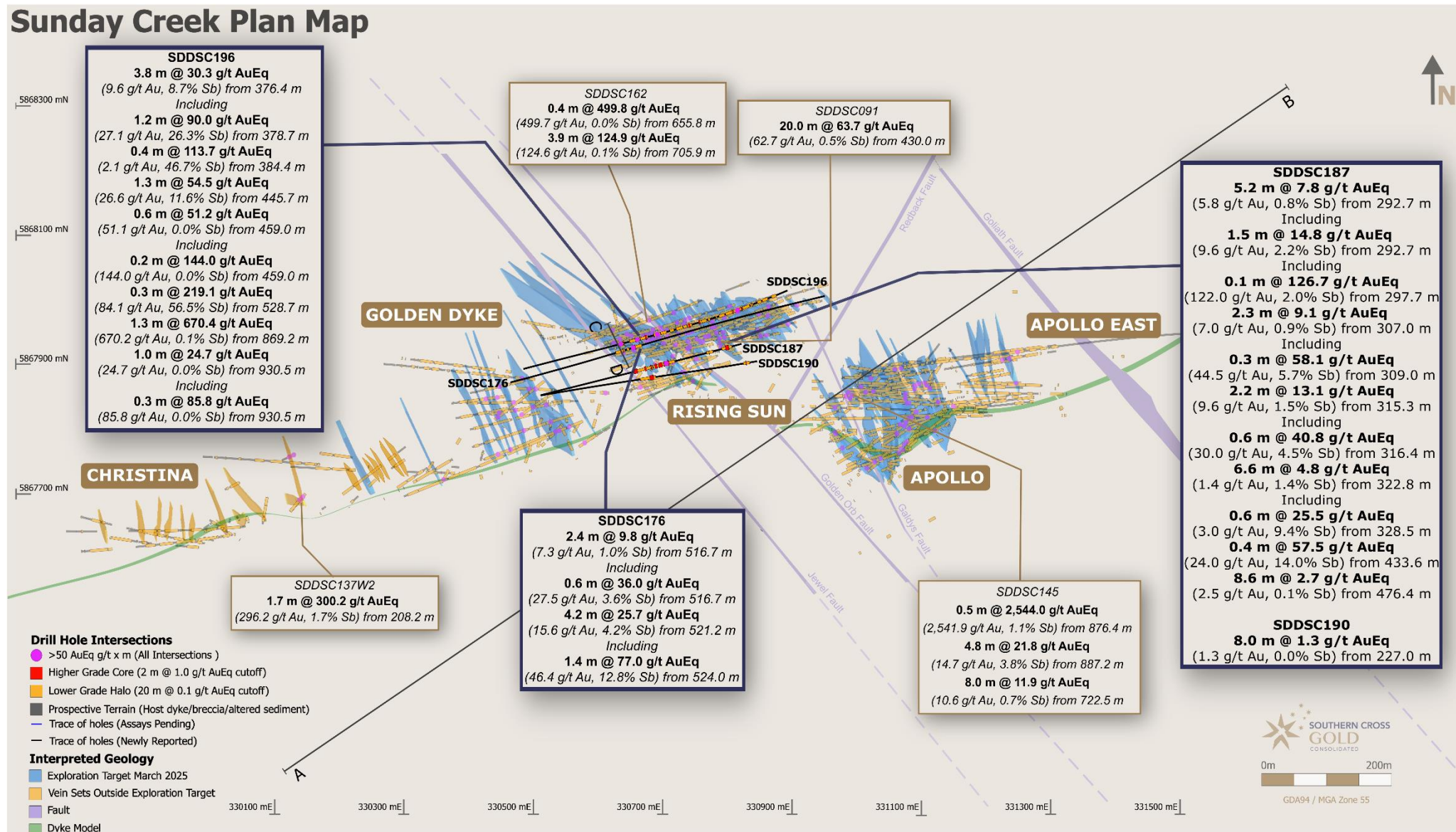
Figure 1: Sunday Creek plan view showing selected results from holes SDDSC176, SDDSC187, SDDSC190 and SDDSC196 reported here (dark blue highlighted box, black trace), with selected prior reported drill holes.
