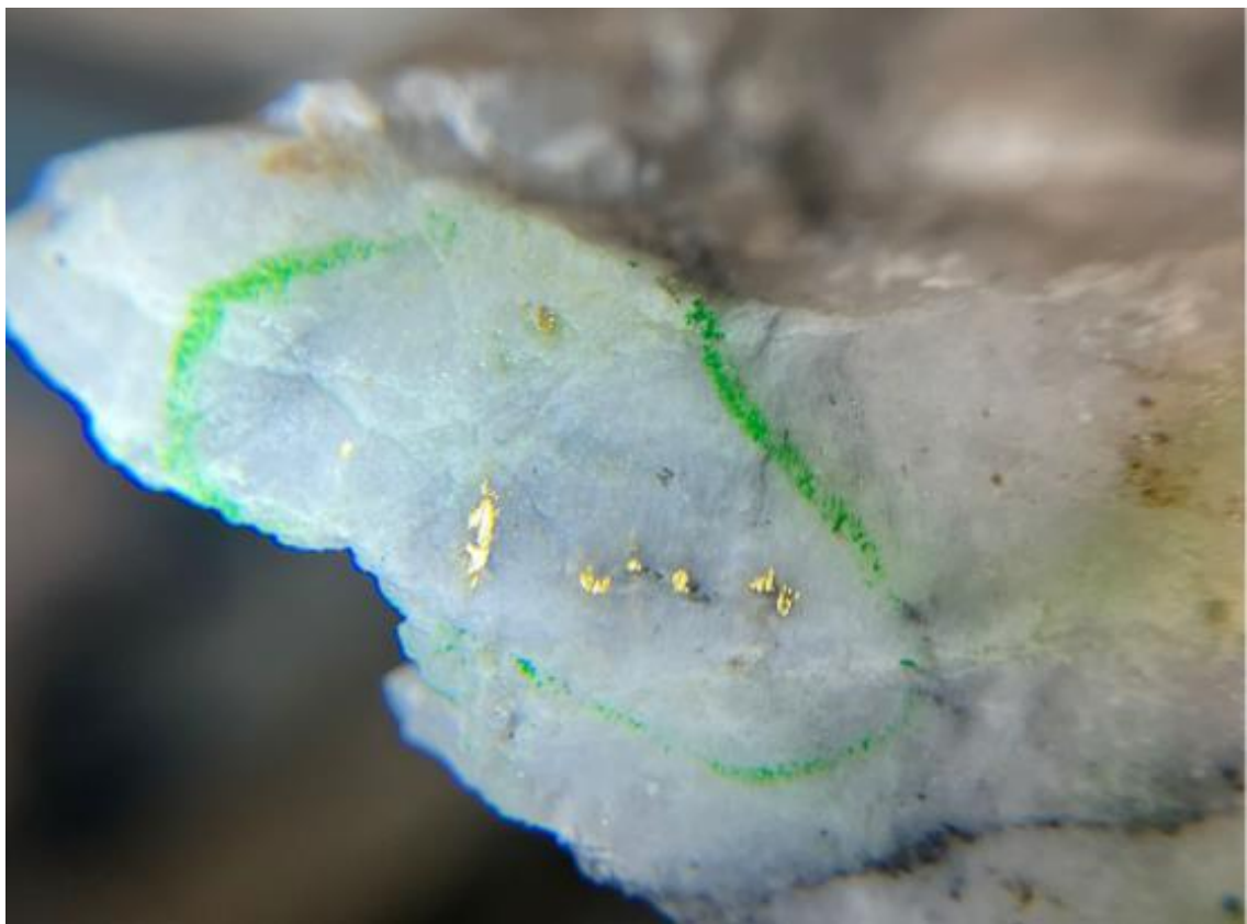
Photos 1 and 2: Visible gold in SDDSC196 in quartz + carbonate +/- stibnite veining from 869.19 m (978 g/t Au, 0.06% Sb). Field of view 2 cm in both images.
