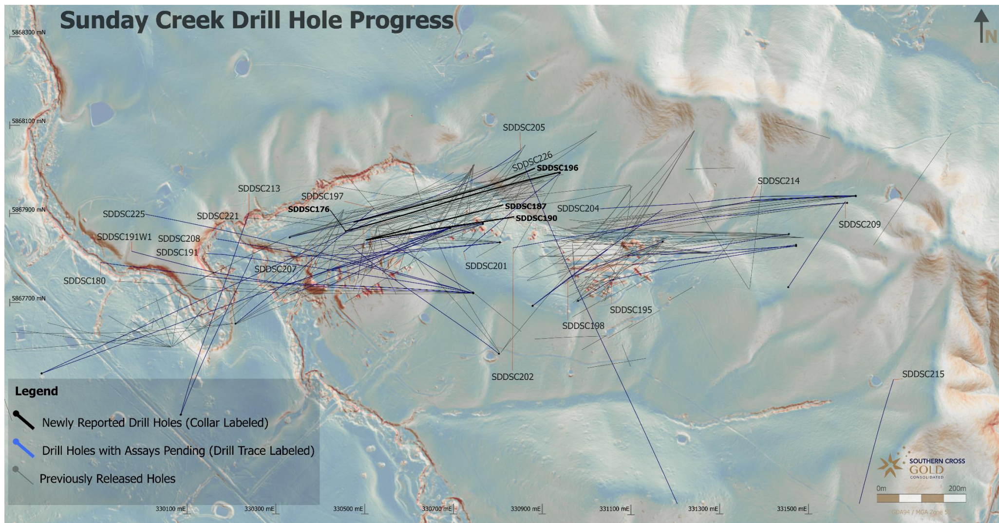
Figure 2: Sunday Creek plan view showing selected drillhole traces from holes SDDSC176, SDDSC187, SDDSC190 and SDDSC196 reported here (black trace), with prior reported drill holes (grey trace) and currently drilling and assays pending hole traces (dark blue).
