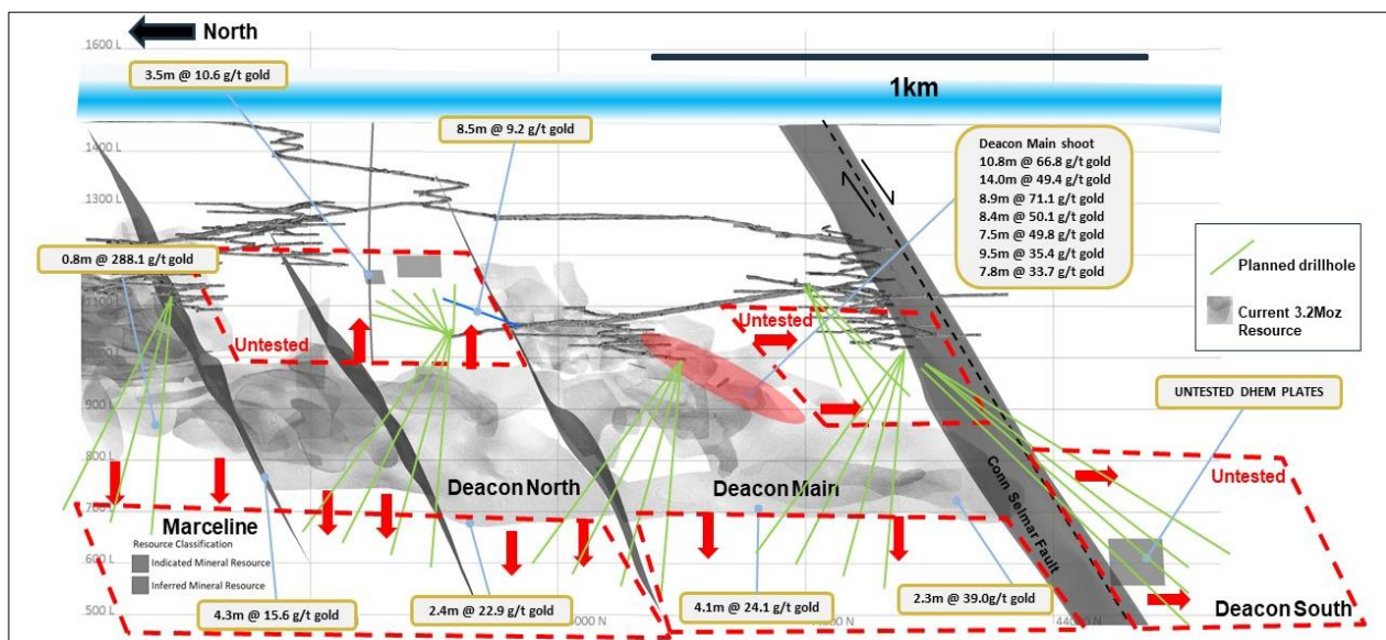
Figure 6: Deacon long section looking east showing current underground position and opportunities for Resource growth from extensions to existing Resource areas. Schematic planned drillholes from existing underground access are shown in green. 17
