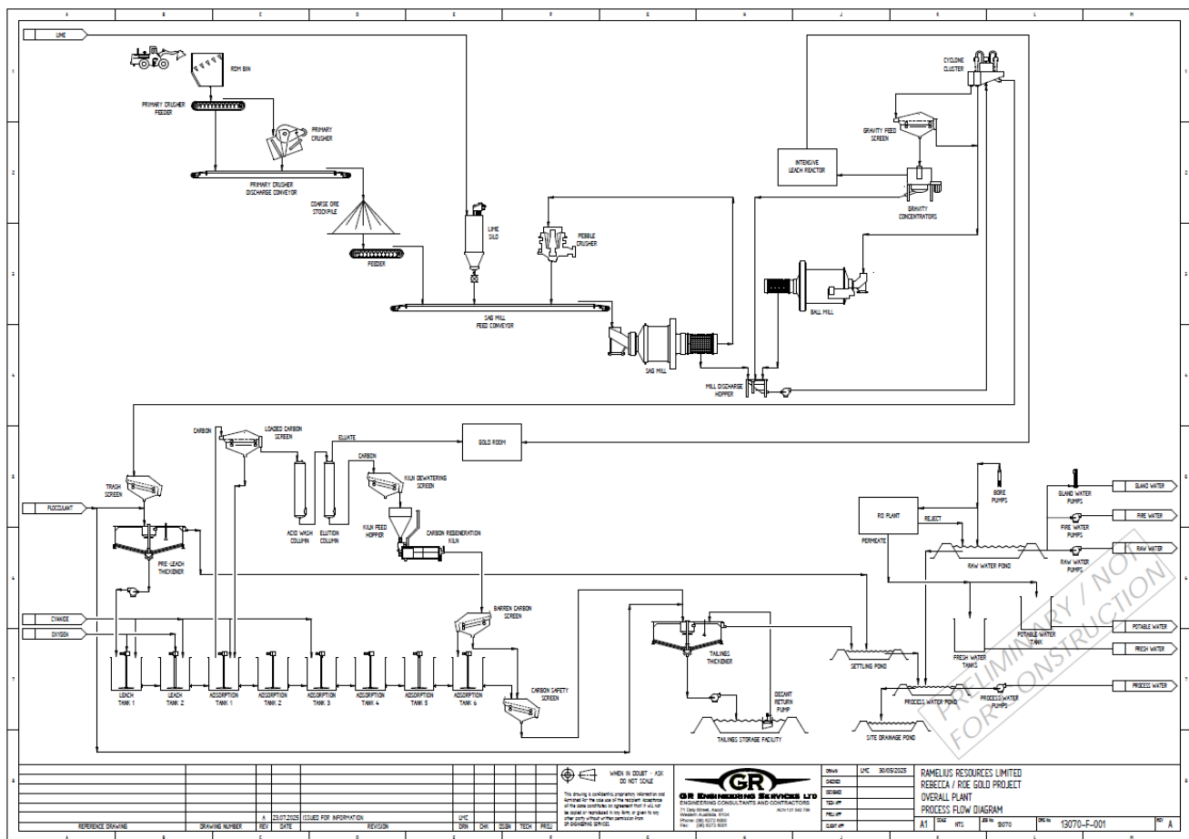
Figure 12: Rebecca process plant process flow diagram
