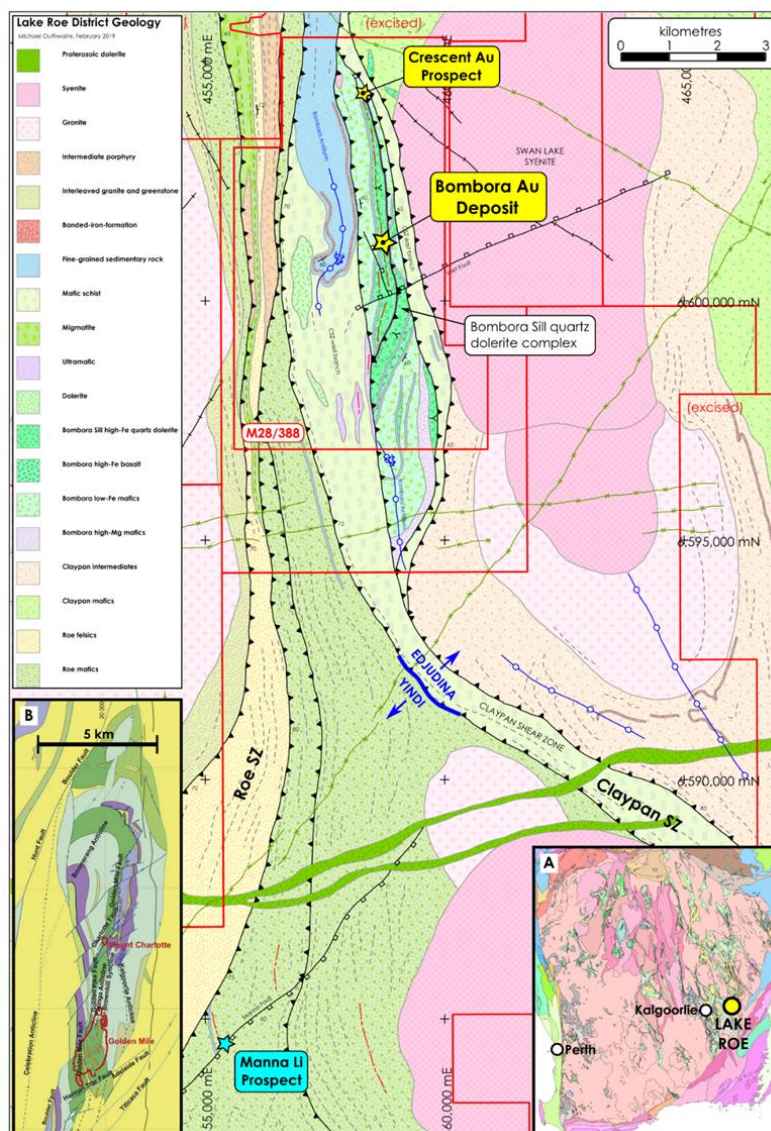
Figure 5: District geology of the Lake Roe project with significant structures (black), GSWA domain boundaries (blue)
