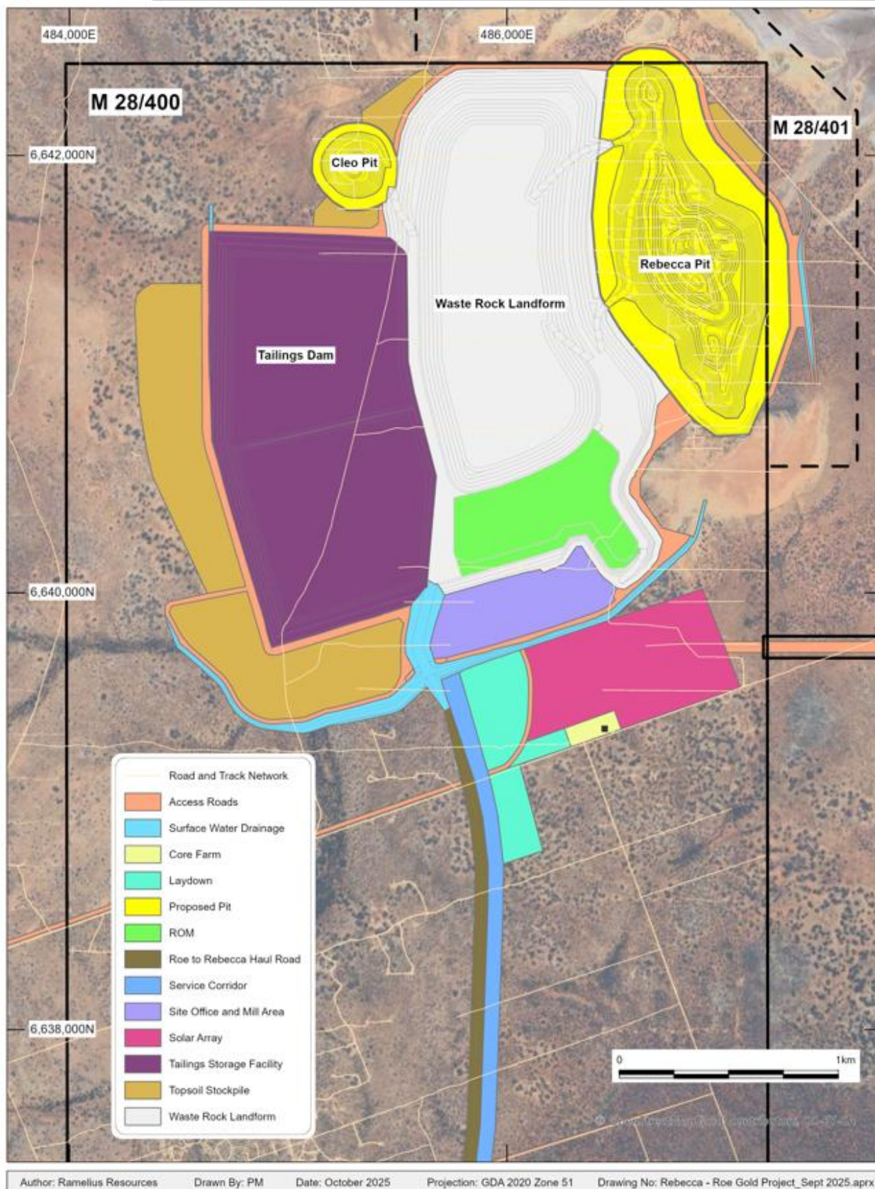
Figure 13: Rebecca TSF and process plant general arrangement
