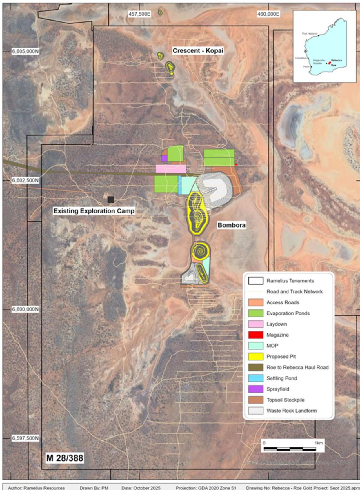
Figure 10: Roe site layout
