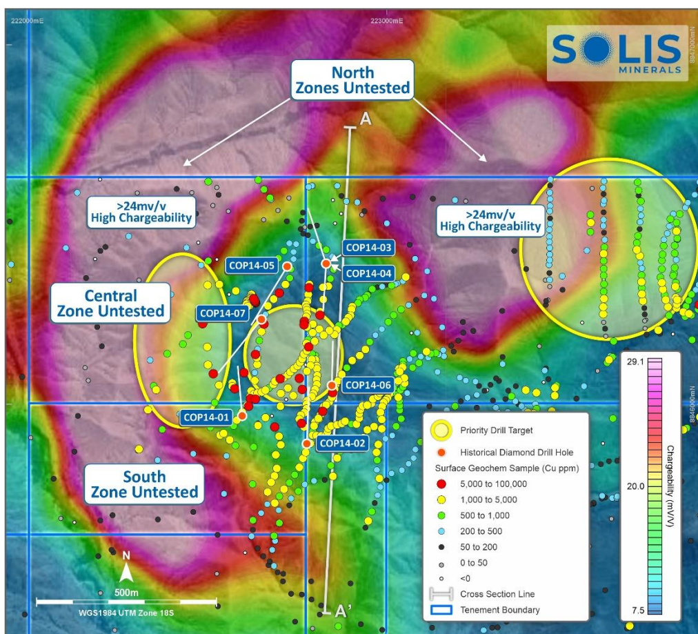
Figure 2: Plan of large geophysical chargeability anomalies at Cucho with drill hole traces overlaid with geochemistry sample assays. Priority drill targets presented. X-section included in Figure 3.
