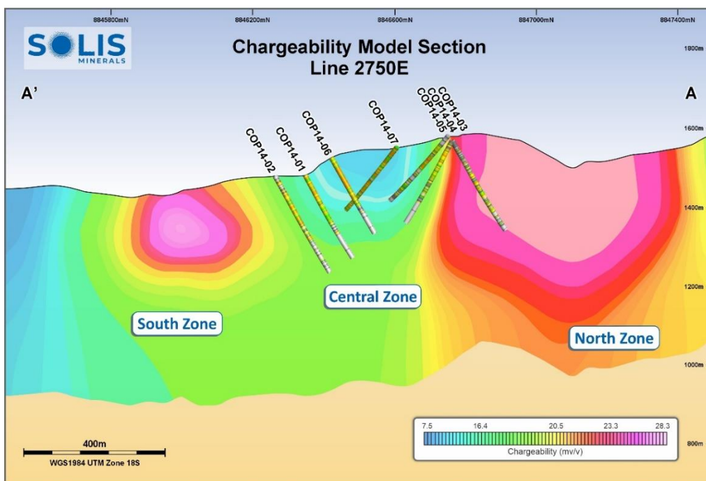
Figure 3: Cucho long section with projection of drill core traces on geophysical IP chargeability anomalies.
