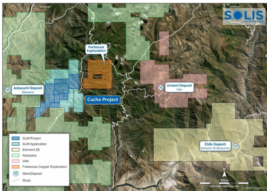
Figure 1: Cucho Project area and surrounding exploration and development projects
