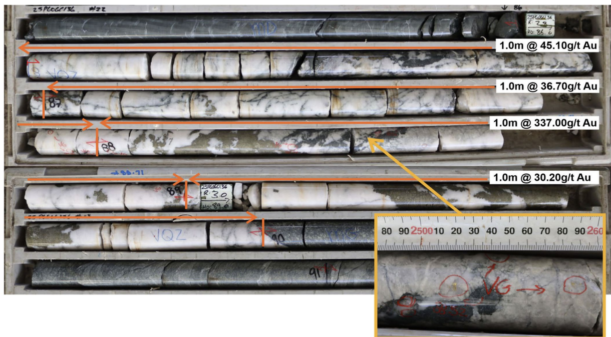
Figure 2: Core Photo of 25PGOGC25136 showing the 5m @ 90.55g/t Au interval with the sub-sample intervals indicated.
